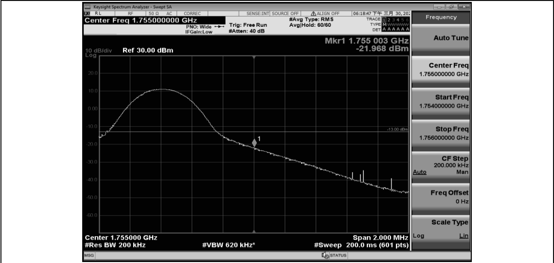
Band4-10MHz-QPSK-20350-50RB#0
