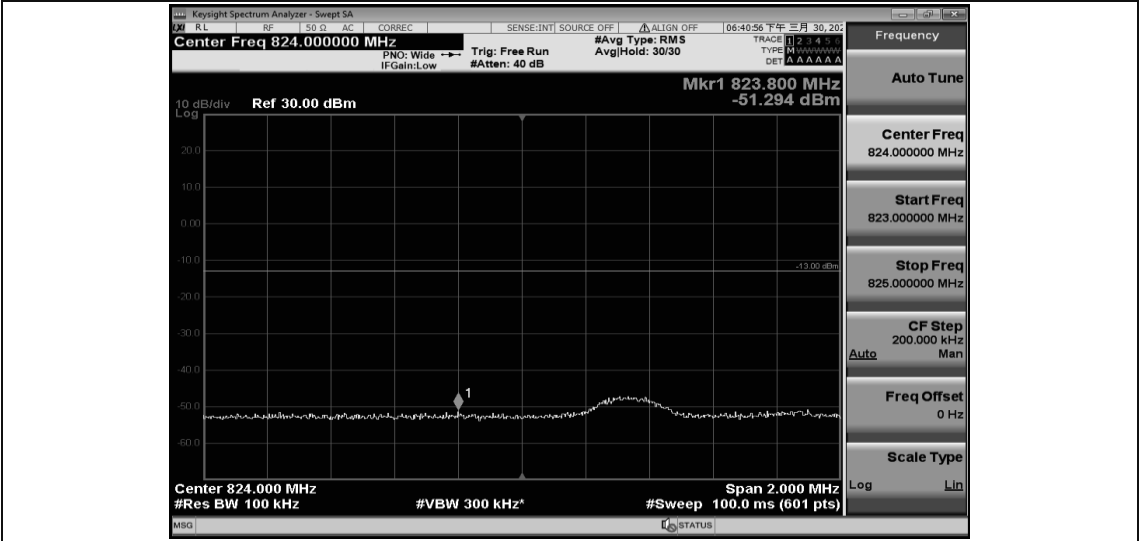
Band5-5MHz-16QAM-20425-25RB#0
