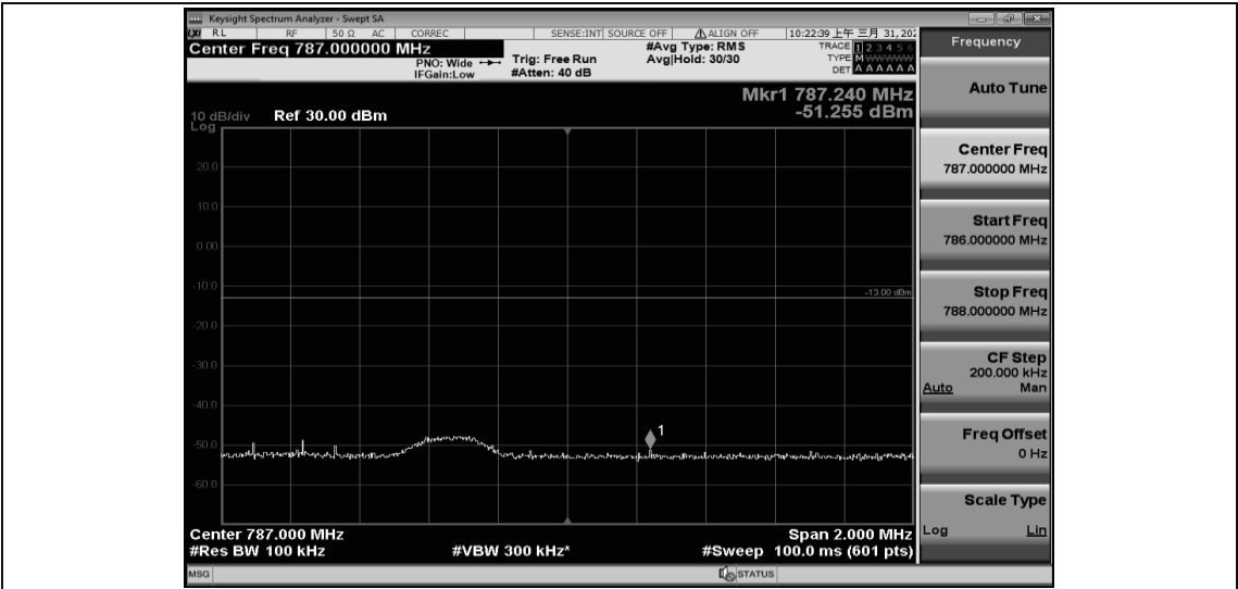
Band13-5MHz-QPSK-23255-1RB#24
