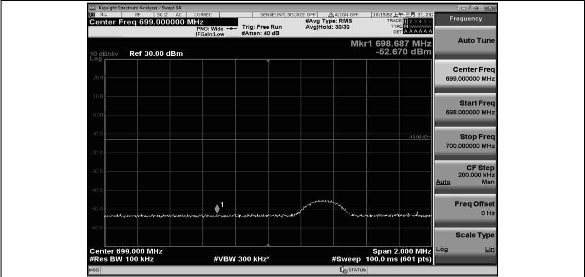
Band12-5MHz-16QAM-23035-1RB#0
