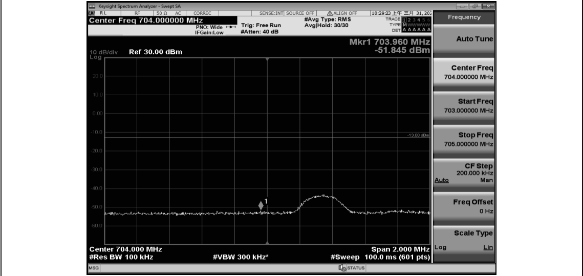
Band17-5MHz-16QAM-23755-25RB#0
