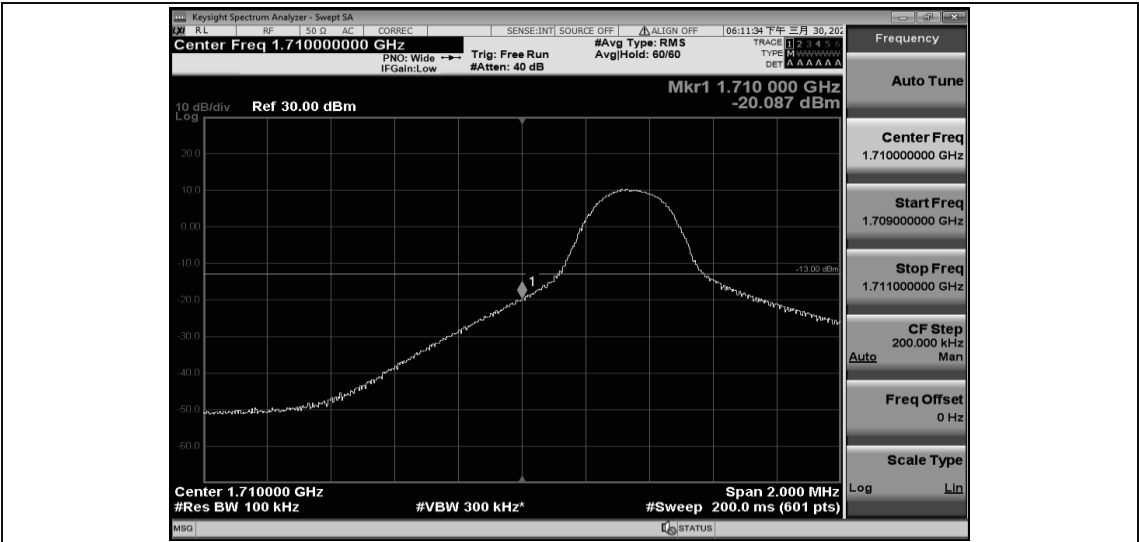
Band4-5MHz-16QAM-19975-1RB#24
