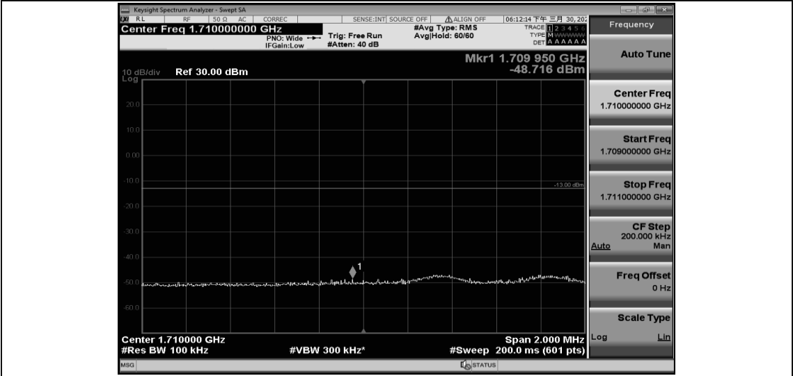
Band4-5MHz-16QAM-19975-25RB#0
