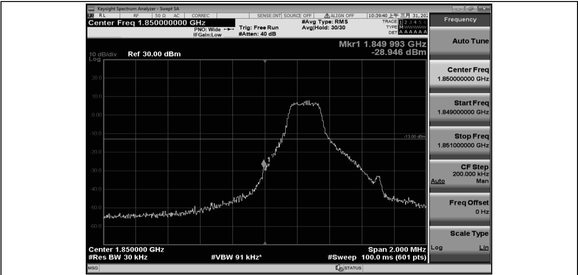
Band25-1.4MHz-16QAM-26047-1RB#5
