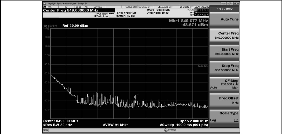
Band5-1.4MHz-QPSK-20643-6RB#0
