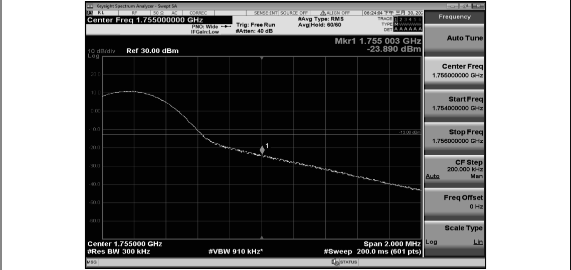
Band4-15MHz-16QAM-20325-75RB#0
