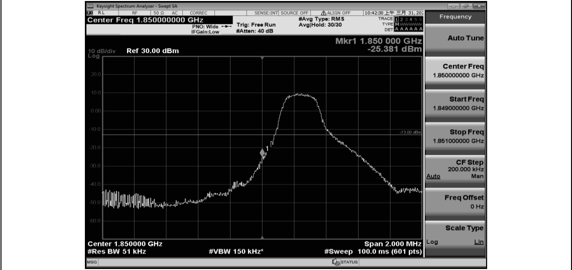
Band25-3MHz-QPSK-26055-15RB#0
