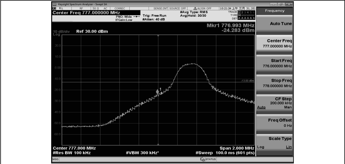
Band13-5MHz-16QAM-23205-25RB#0
