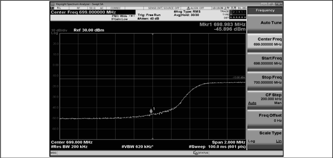
Band12-10MHz-16QAM-23130-1RB#49
