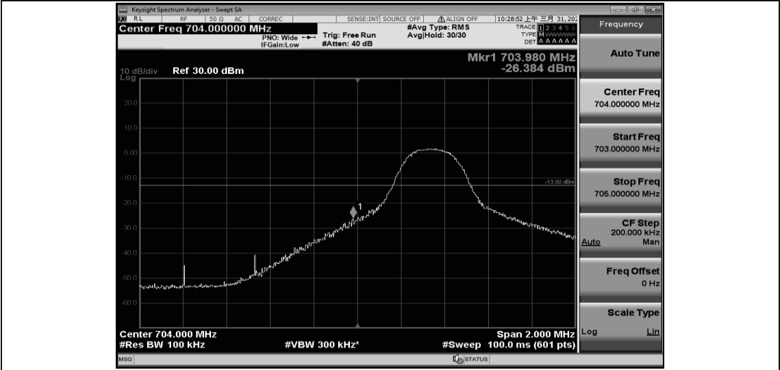
Band17-5MHz-QPSK-23755-25RB#0
