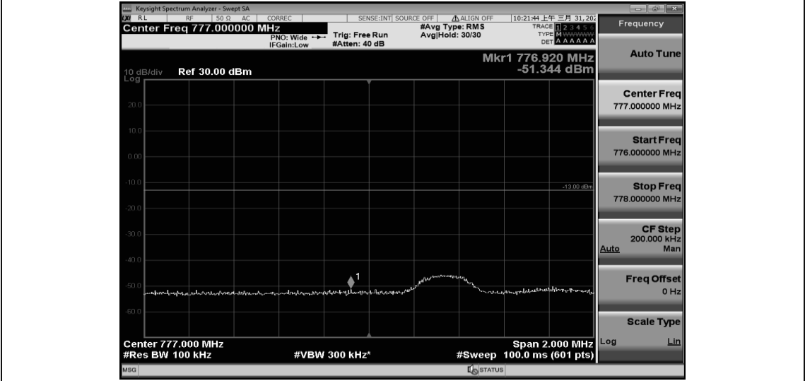
Band13-5MHz-QPSK-23205-25RB#0
