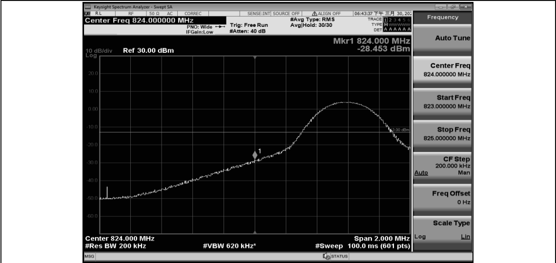
Band5-10MHz-QPSK-20450-50RB#0
