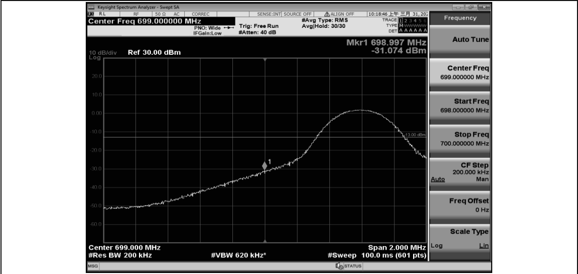
Band12-10MHz-QPSK-23060-50RB#0
