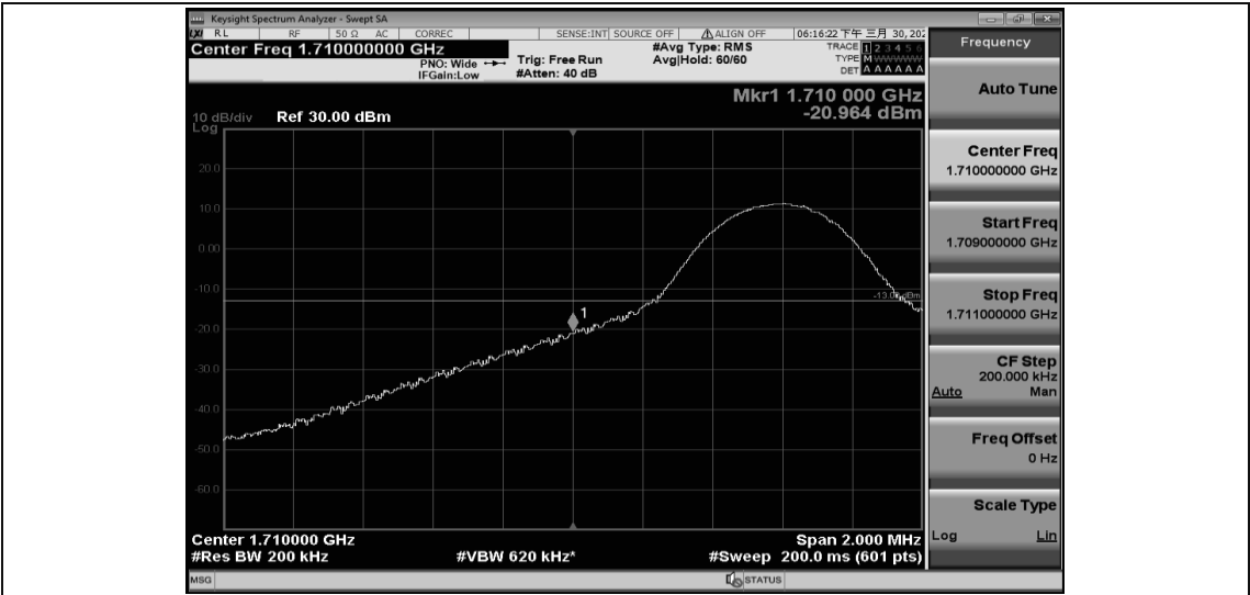
Band4-10MHz-16QAM-20000-1RB#49
