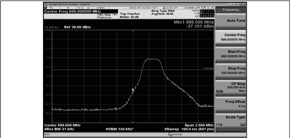
Band12-3MHz-QPSK-23025-1RB#14
