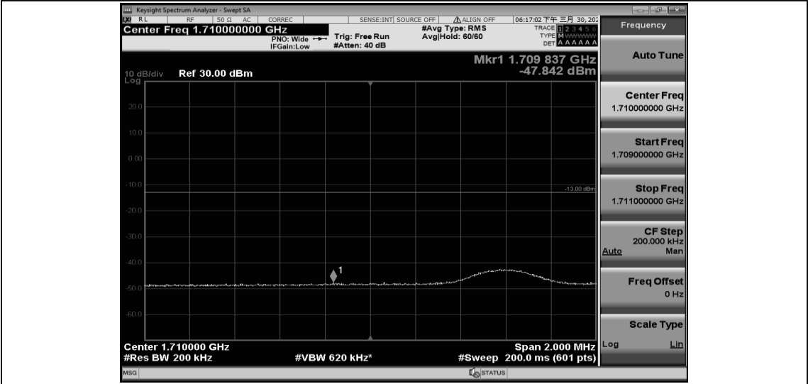
Band4-10MHz-16QAM-20000-50RB#0
