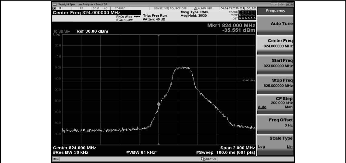
Band5-1.4MHz-QPSK-20407-6RB#0
