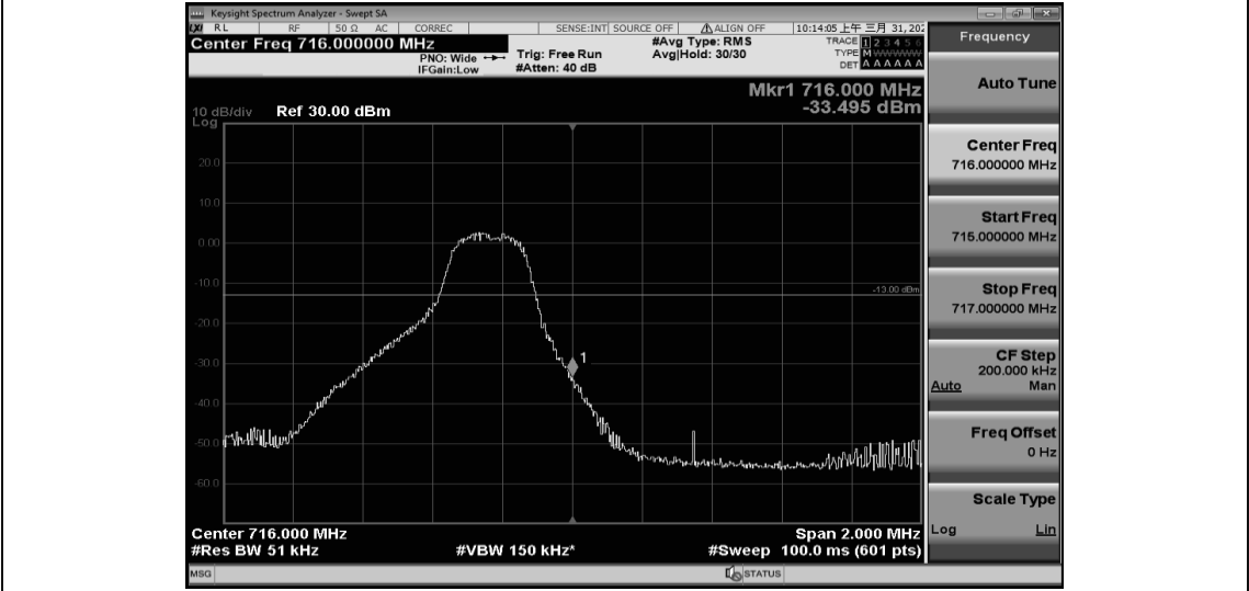
Band12-3MHz-16QAM-23165-15RB#0
