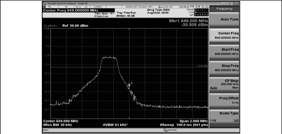
Band5-1.4MHz-16QAM-20643-6RB#0
