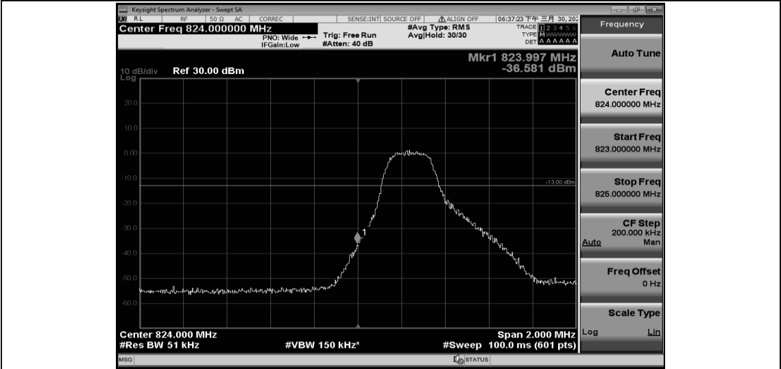
Band5-3MHz-16QAM-20415-15RB#0
