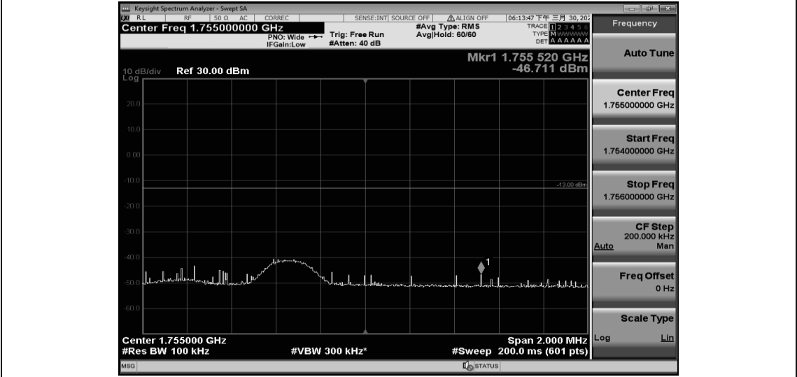
Band4-5MHz-16QAM-20375-25RB#0
