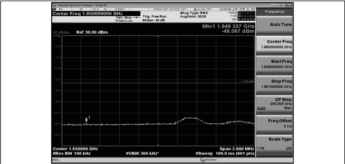
Band25-5MHz-QPSK-26065-1RB#0
