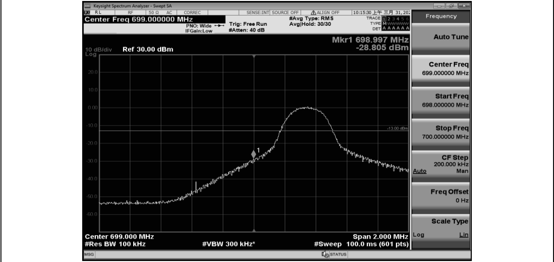
Band12-5MHz-16QAM-23035-25RB#0
