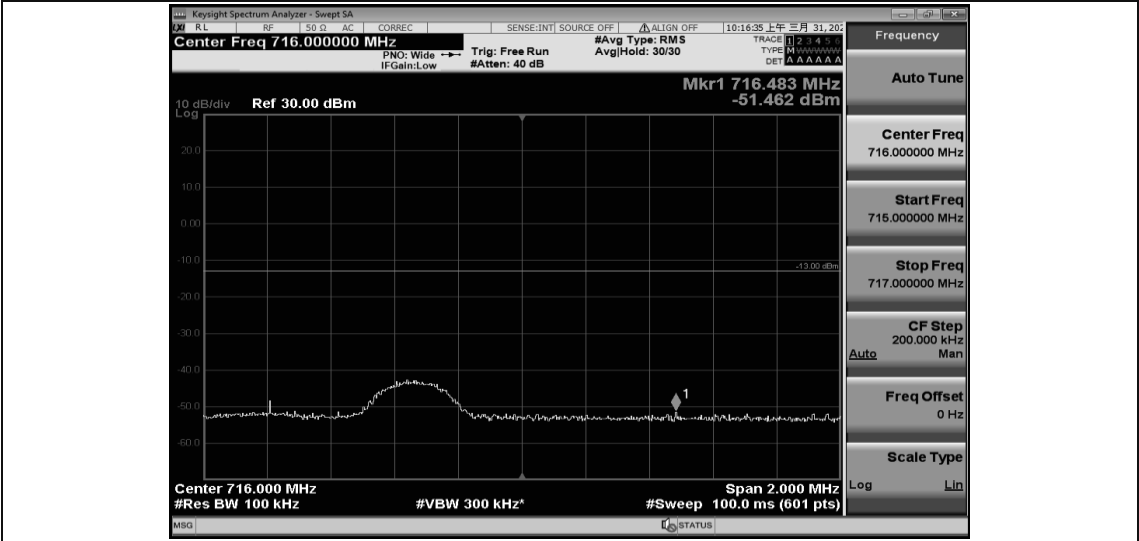
Band12-5MHz-QPSK-23155-25RB#0
