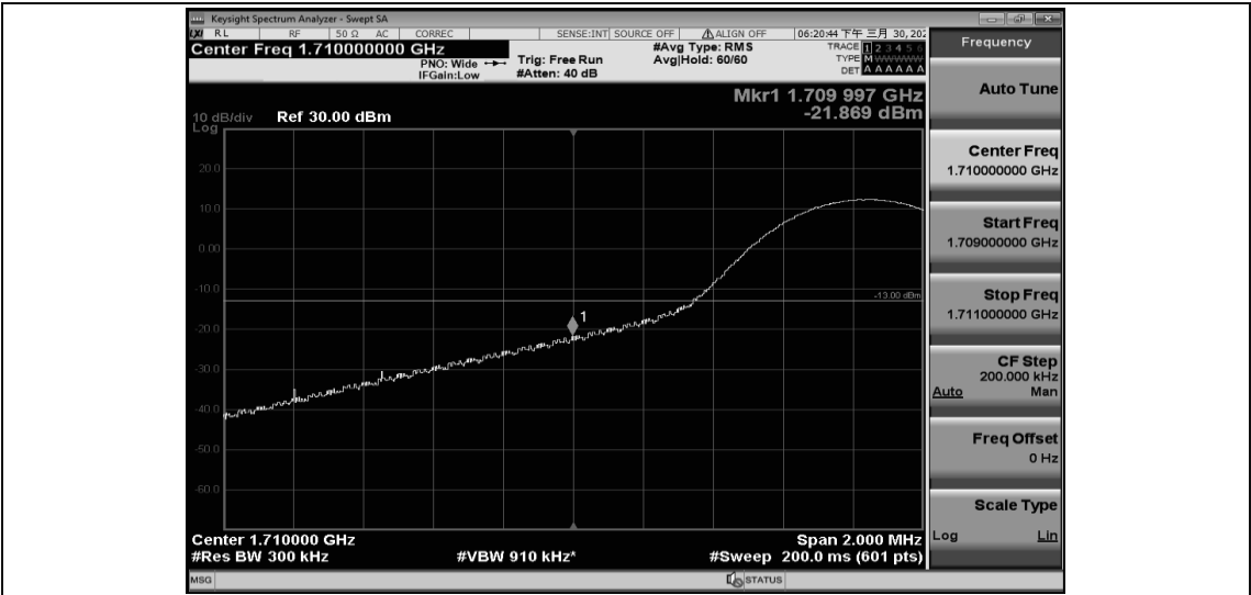
Band4-15MHz-QPSK-20025-1RB#74
