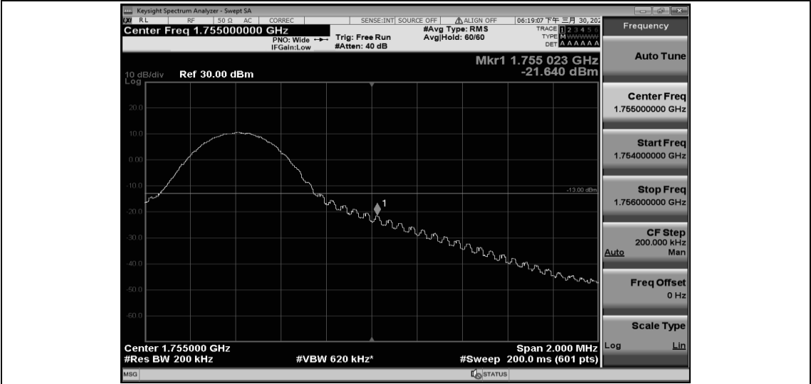
Band4-10MHz-16QAM-20350-1RB#0
