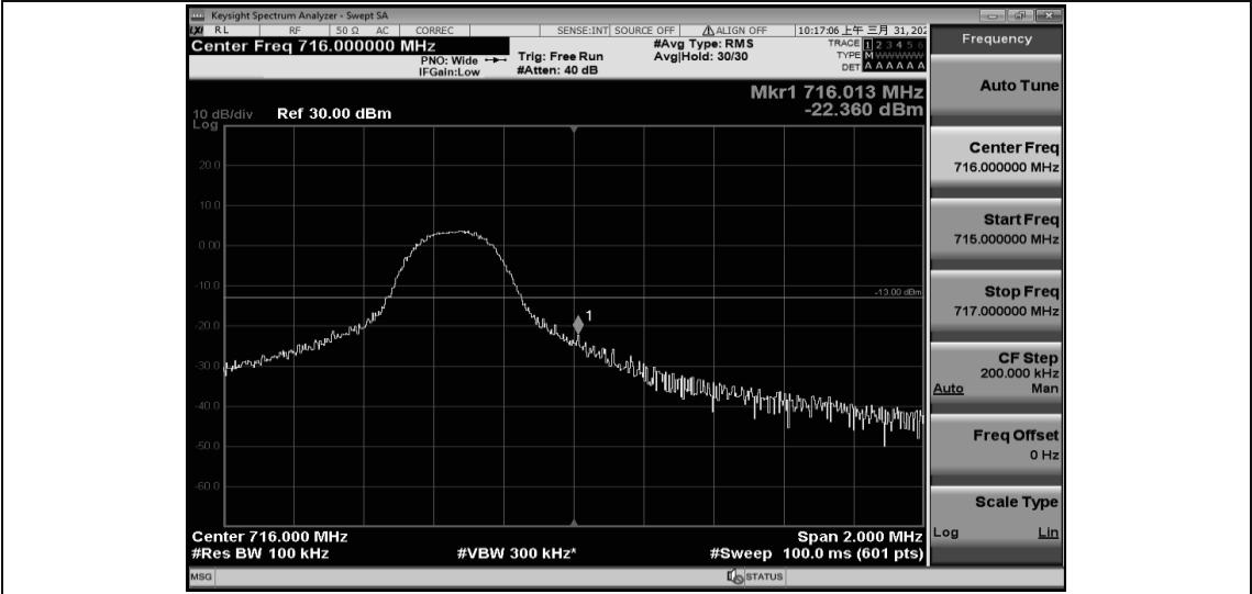
Band12-5MHz-16QAM-23155-25RB#0
