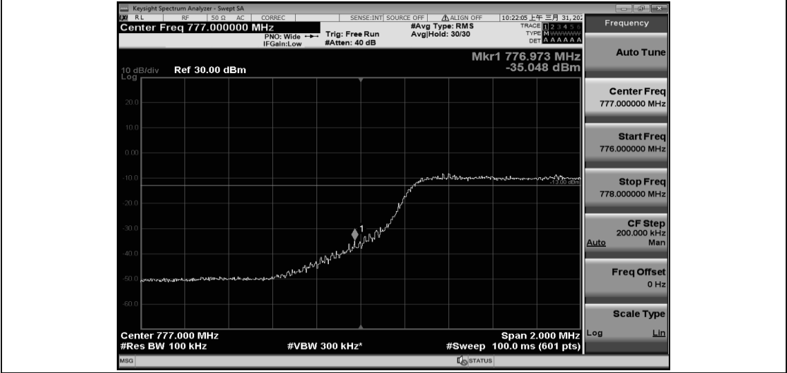
Band13-5MHz-QPSK-23255-1RB#0
