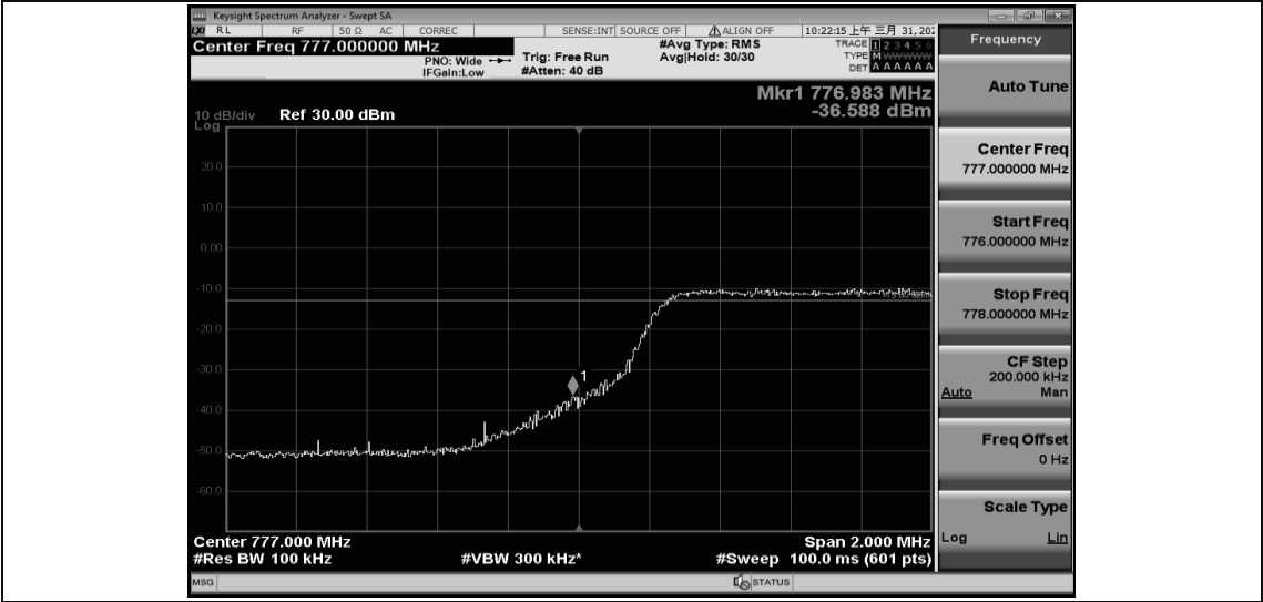
Band13-5MHz-16QAM-23255-1RB#24
