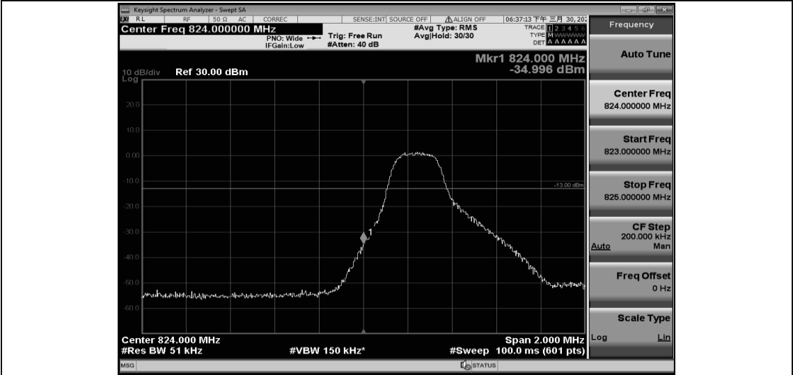
Band5-3MHz-QPSK-20415-15RB#0
