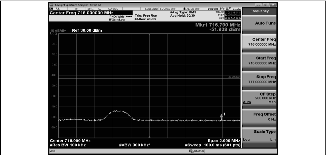
Band12-5MHz-16QAM-23155-1RB#24
