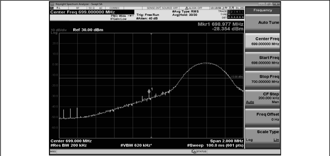
Band12-10MHz-16QAM-23060-50RB#0
