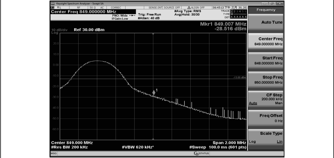
Band5-10MHz-QPSK-20600-50RB#0
