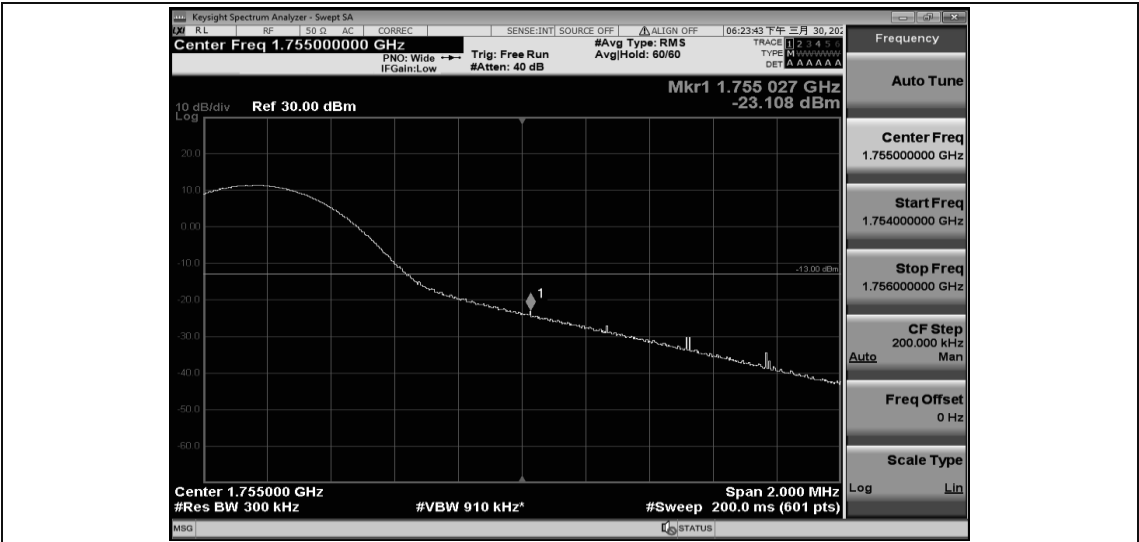
Band4-15MHz-QPSK-20325-1RB#0
