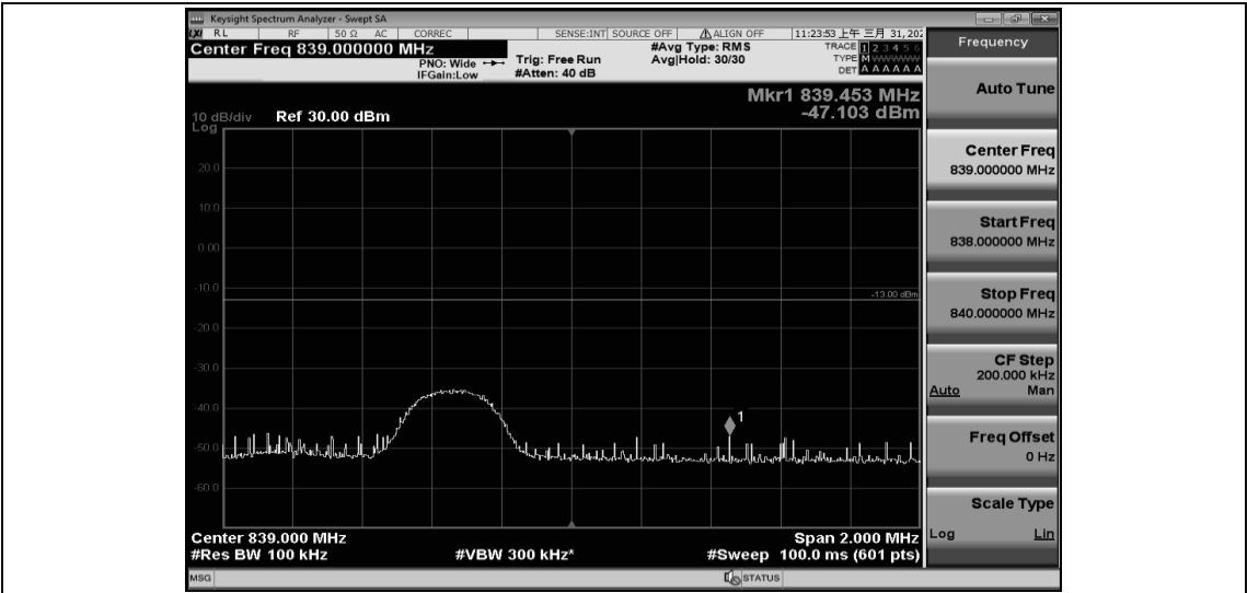
Band26-5MHz-QPSK-26915-1RB#24
