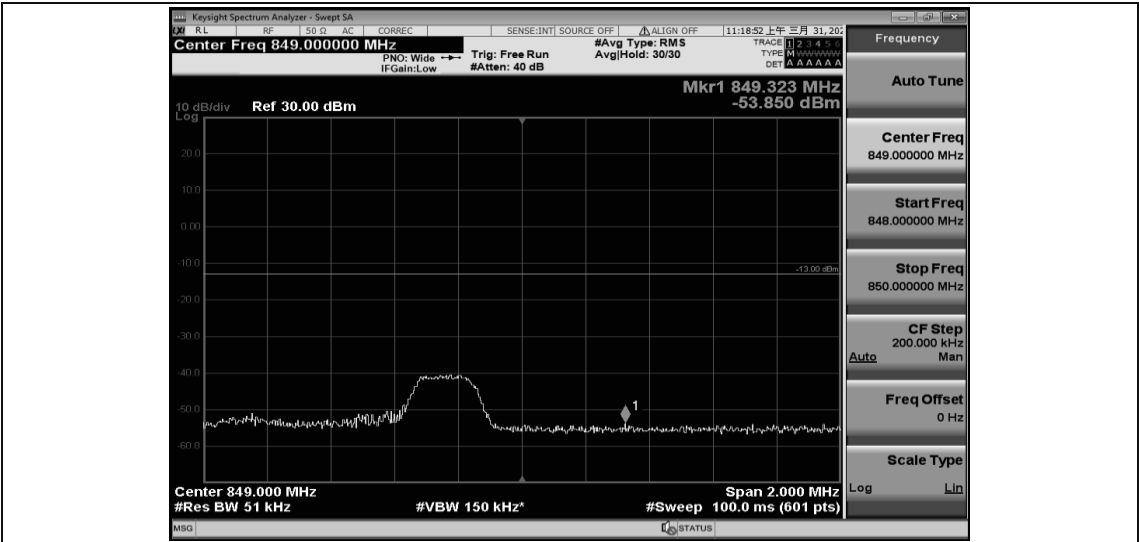
Band26-3MHz-QPSK-27025-1RB#14
