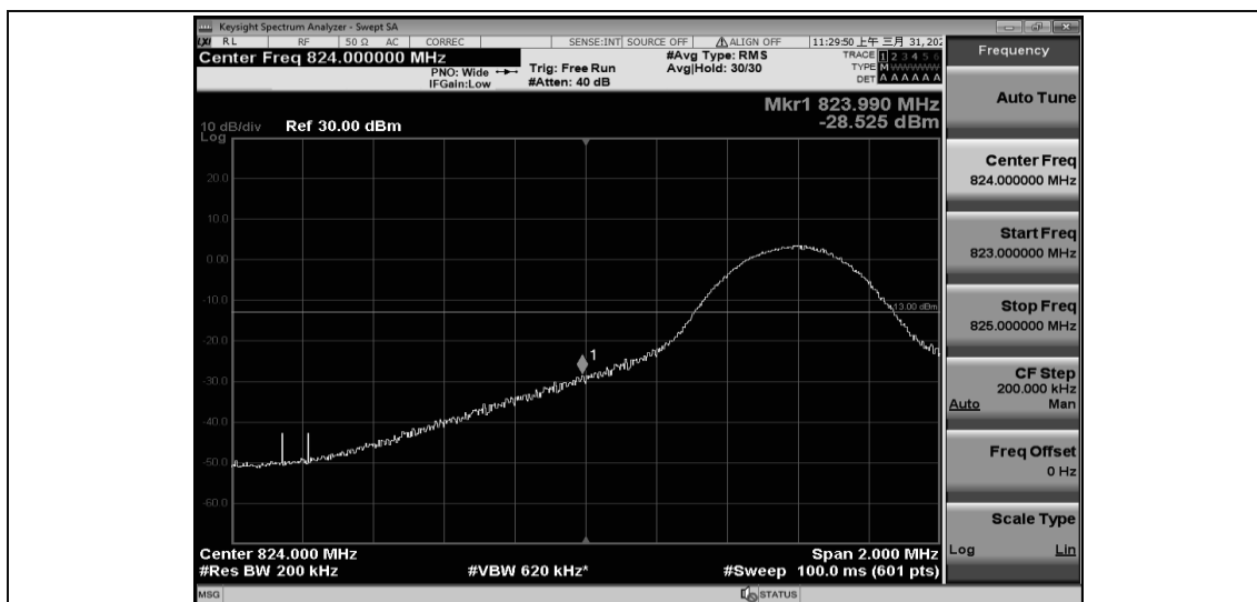
Band26-10MHz-16QAM-26840-1RB#49
