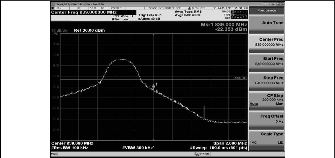
Band26-5MHz-QPSK-26915-25RB#0
