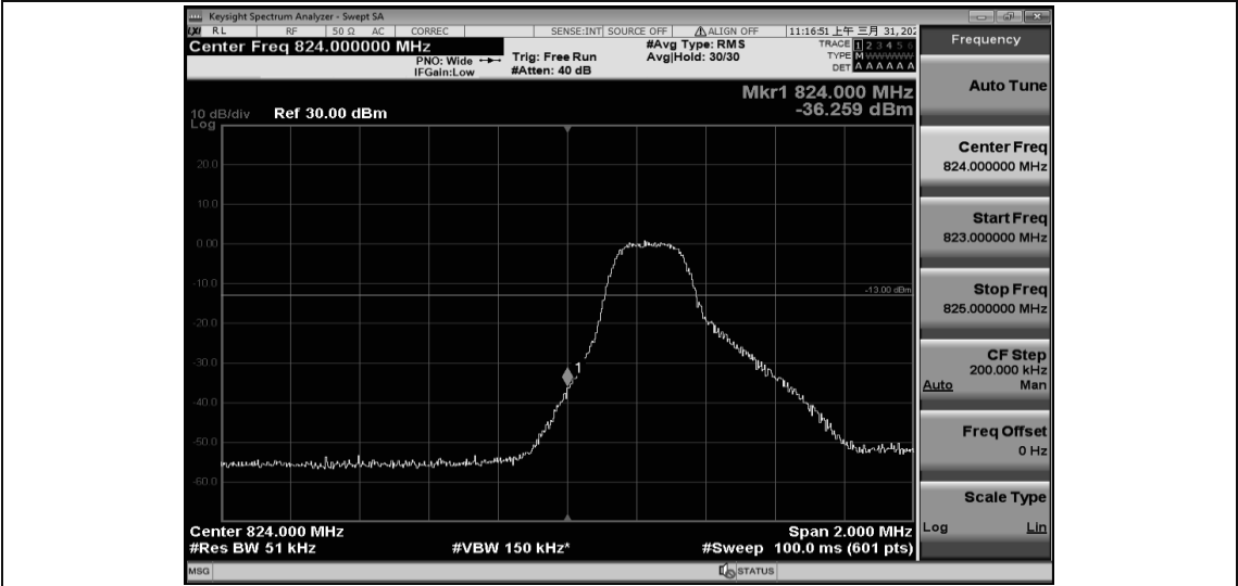
Band26-3MHz-16QAM-26805-1RB#14
