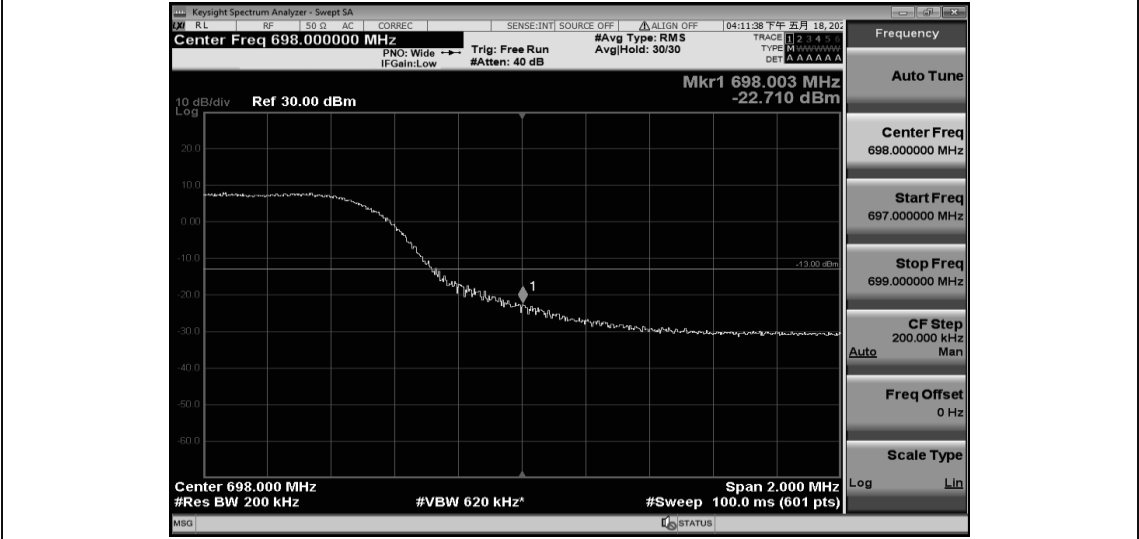
Band71-15MHz-QPSK-133197-75RB#0
