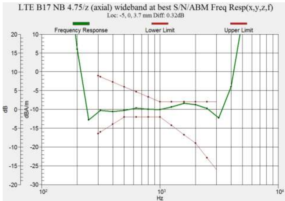
Figure B.14 Frequency Response of LTE Band 17
