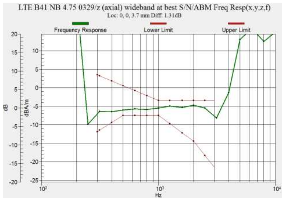
Figure B.19 Frequency Response of LTE Band 41
