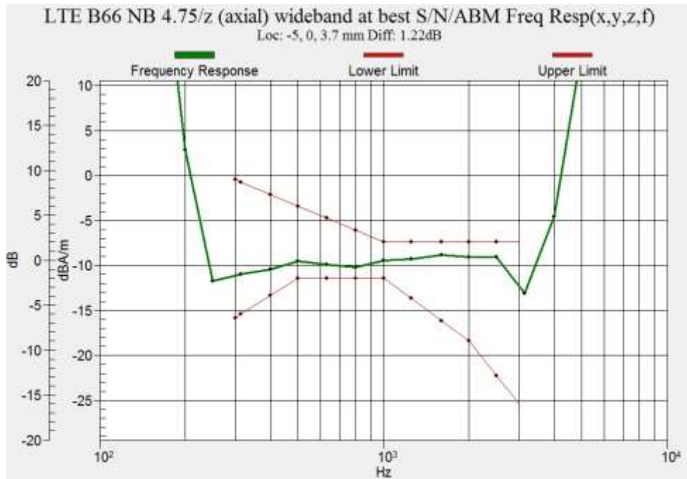
Figure B.17 Frequency Response of LTE Band 66
