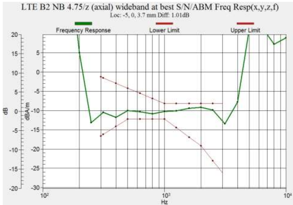
Figure B.9 Frequency Response of LTE Band 2
