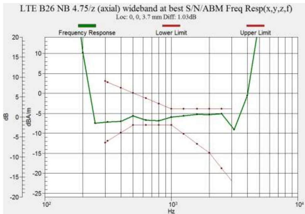
Figure B.16 Frequency Response of LTE Band 26
