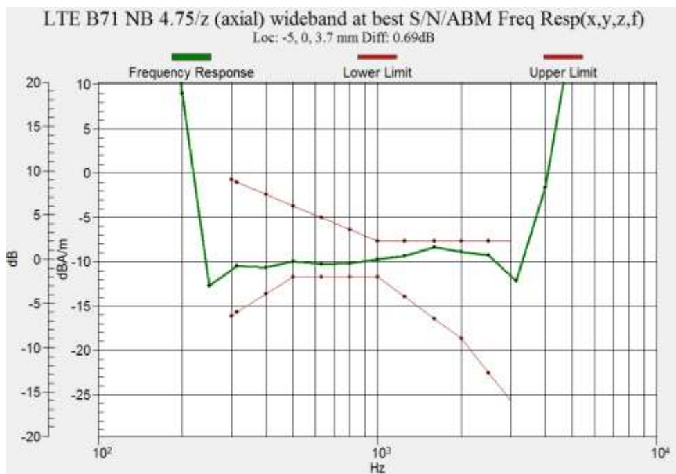
Figure B.18 Frequency Response of LTE Band 71
