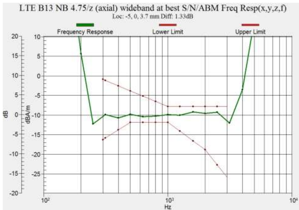
Figure B.13 Frequency Response of LTE Band 13
