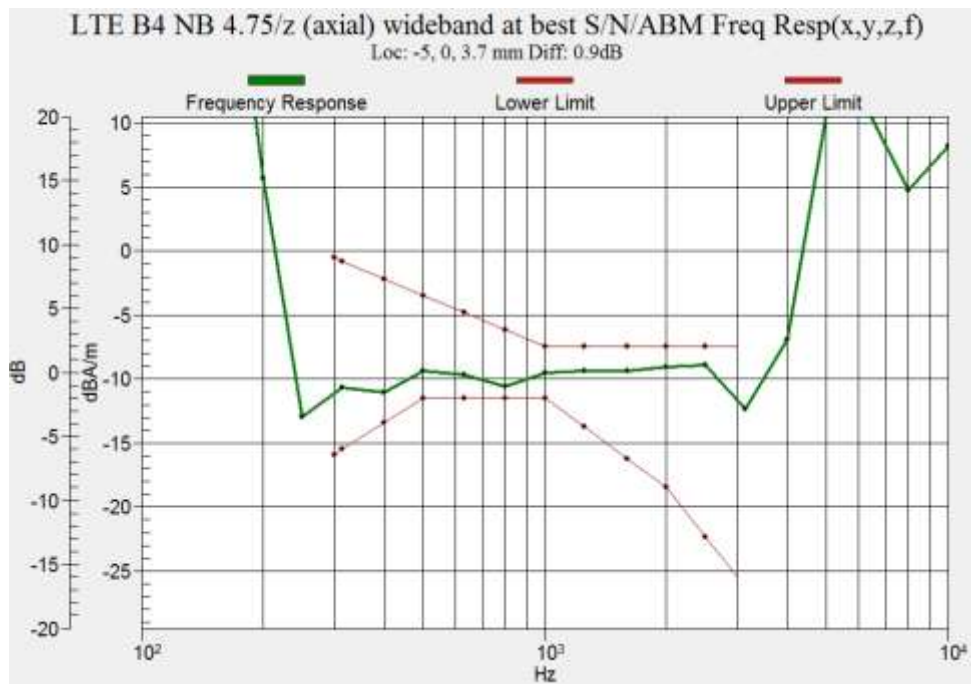
Figure B.10 Frequency Response of LTE Band 4
