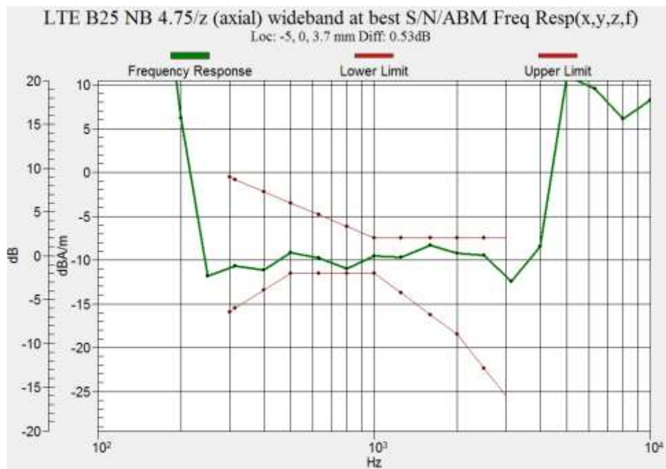
Figure B.15 Frequency Response of LTE Band 25
