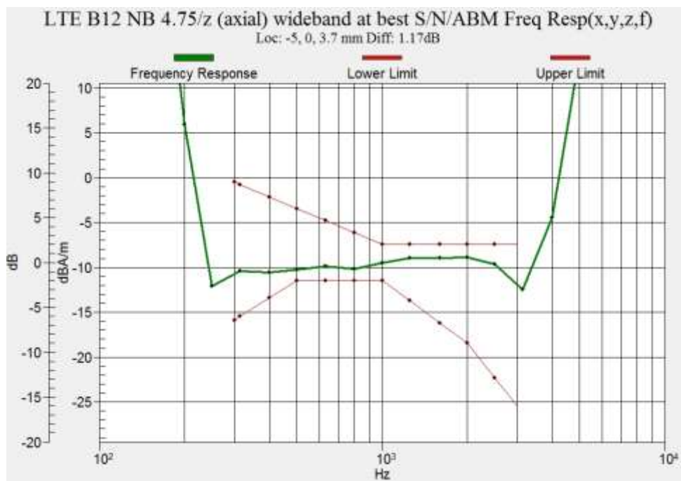
Figure B.12 Frequency Response of LTE Band 12
