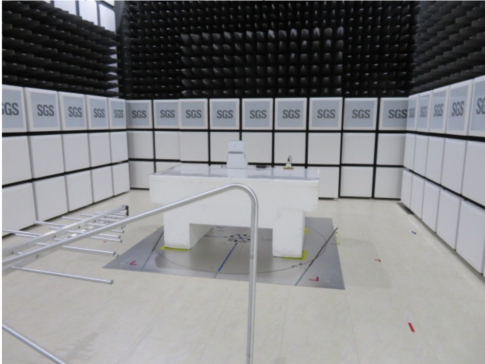
Radiated Emissions (30MHz – 1000MHz) Test Setup
