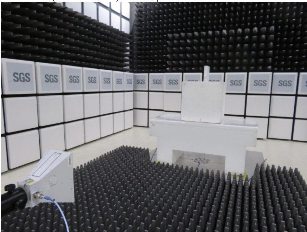
Radiated Emissions (Above 1000MHz) Test Setup
