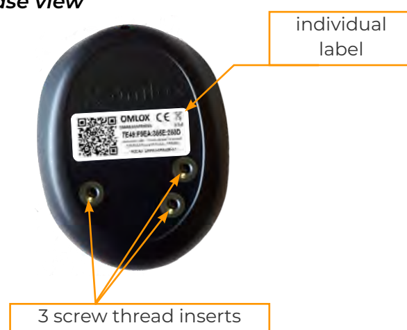
base view
