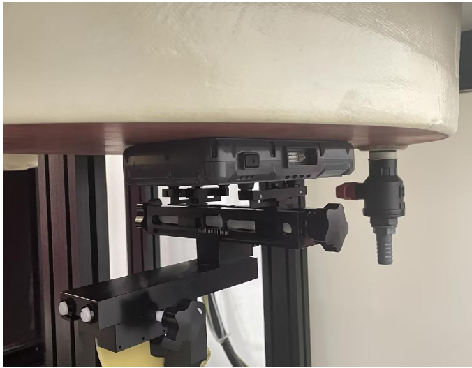
Photo 5: Back Side 0mm
