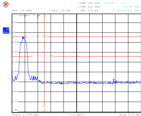
No-hopping mode
