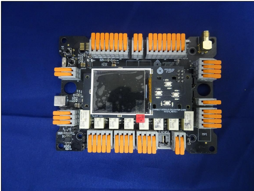
Picture 1 PCB Front View
