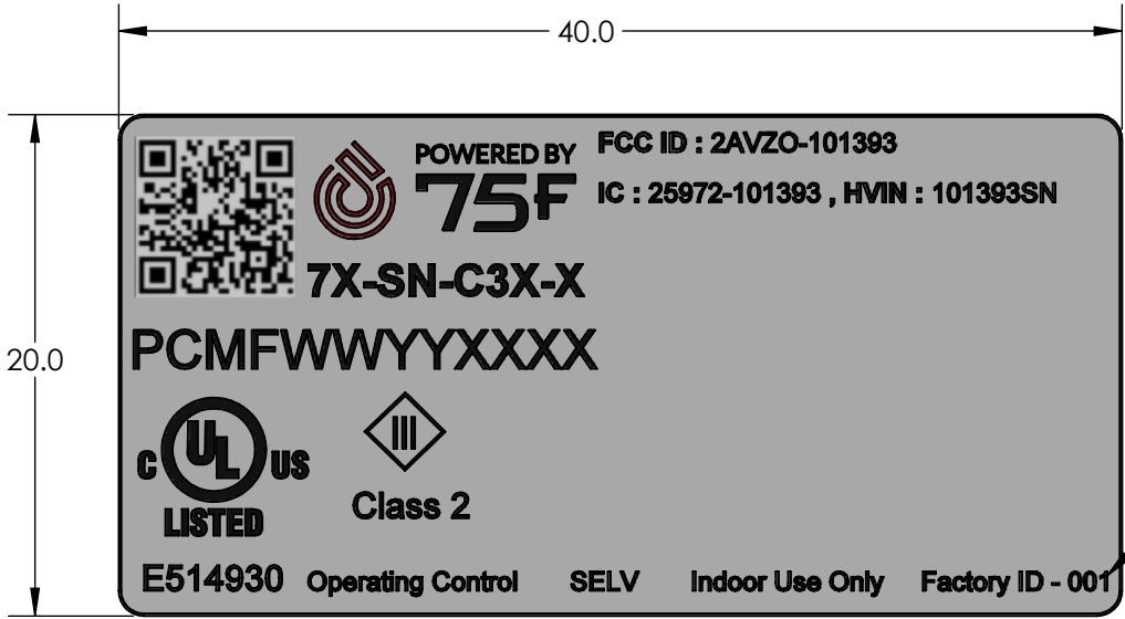
FRONT VIEW SCALE 3:1
