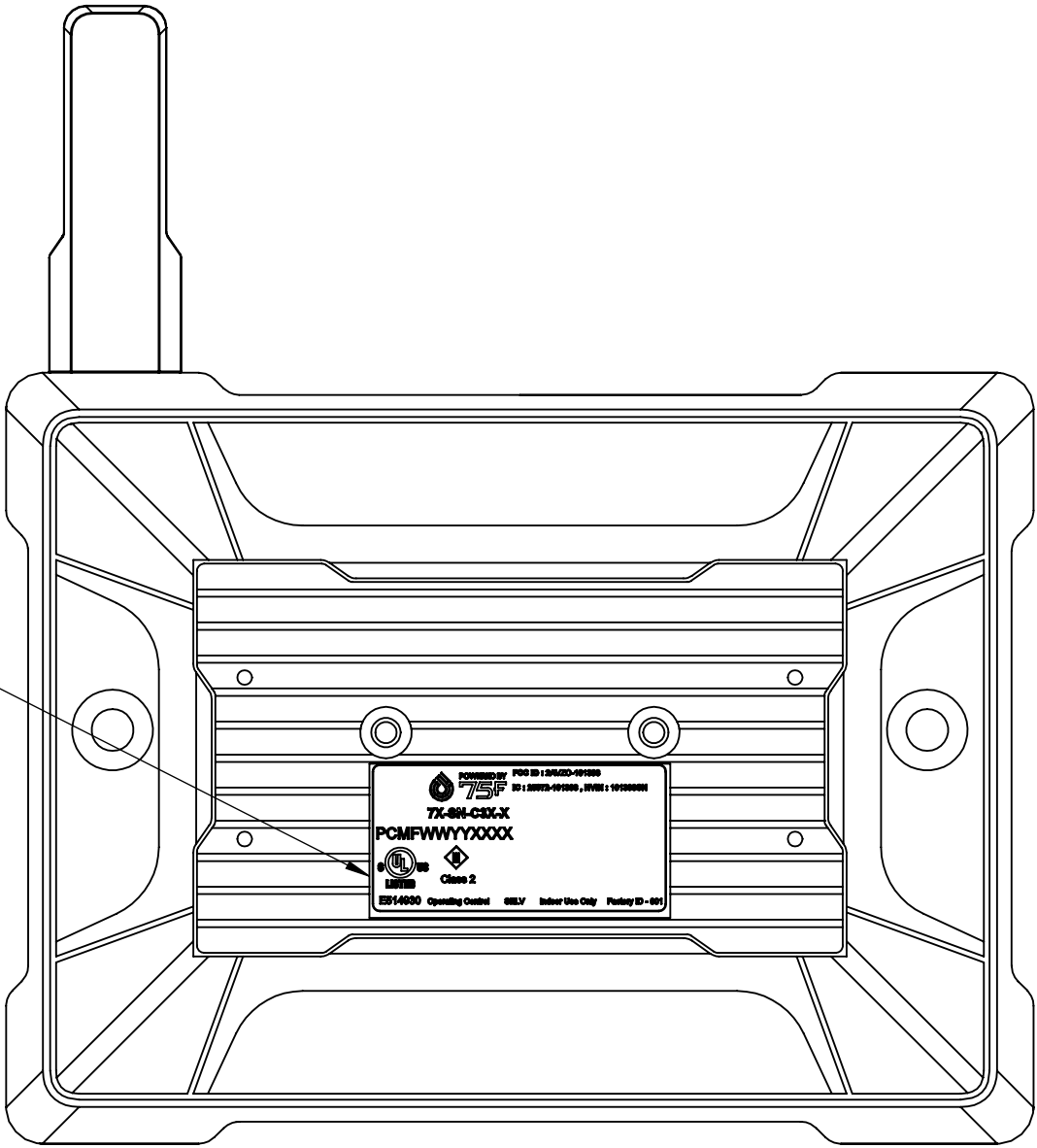
BACK VIEW (VIEW INCLUDED FOR PLACEMENT ONLY) SCALE 1:1
