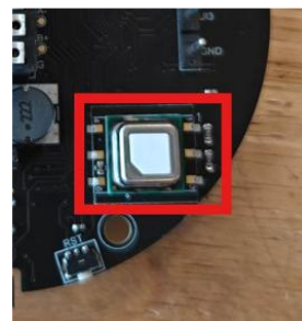
Figure 2: PCB Bottom side (with CO2 sensor mounted – red marked)
