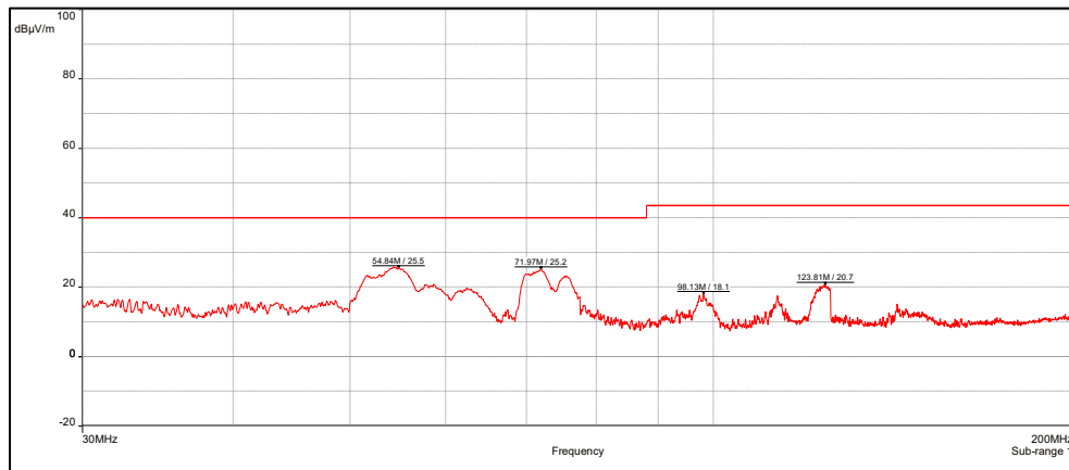
Channel Frequency 30MHz – 200MHz
