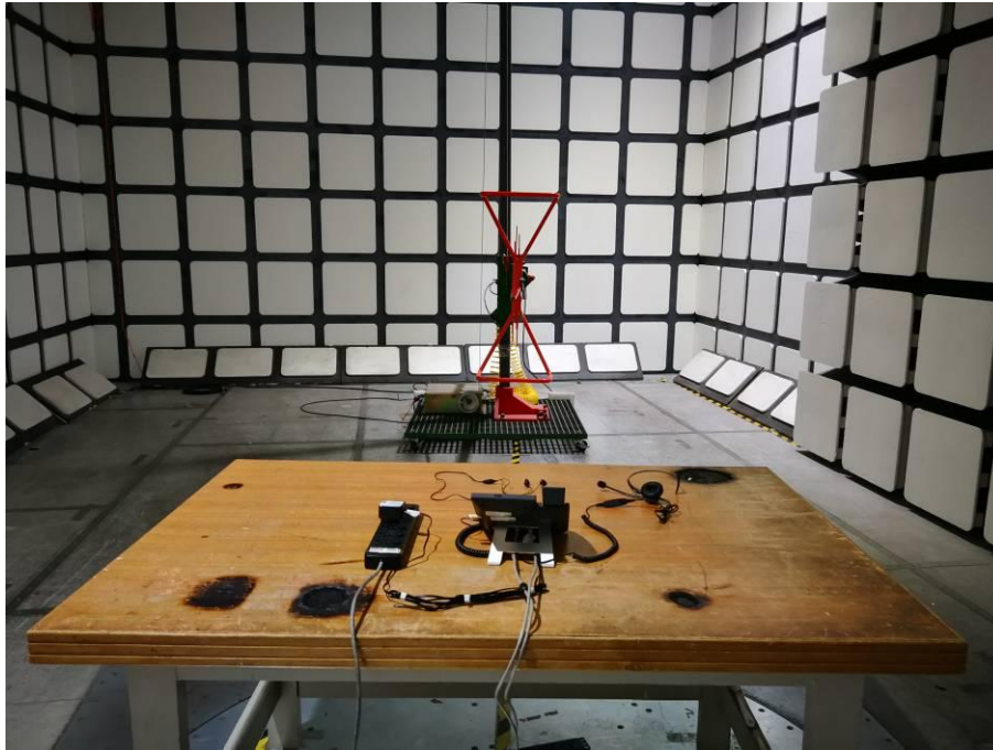
Radiated Emissions View (Below 1 GHz, Powered by adapter)
