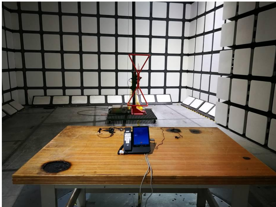
Radiated Emissions View (Below 1 GHz, Powered by POE)
