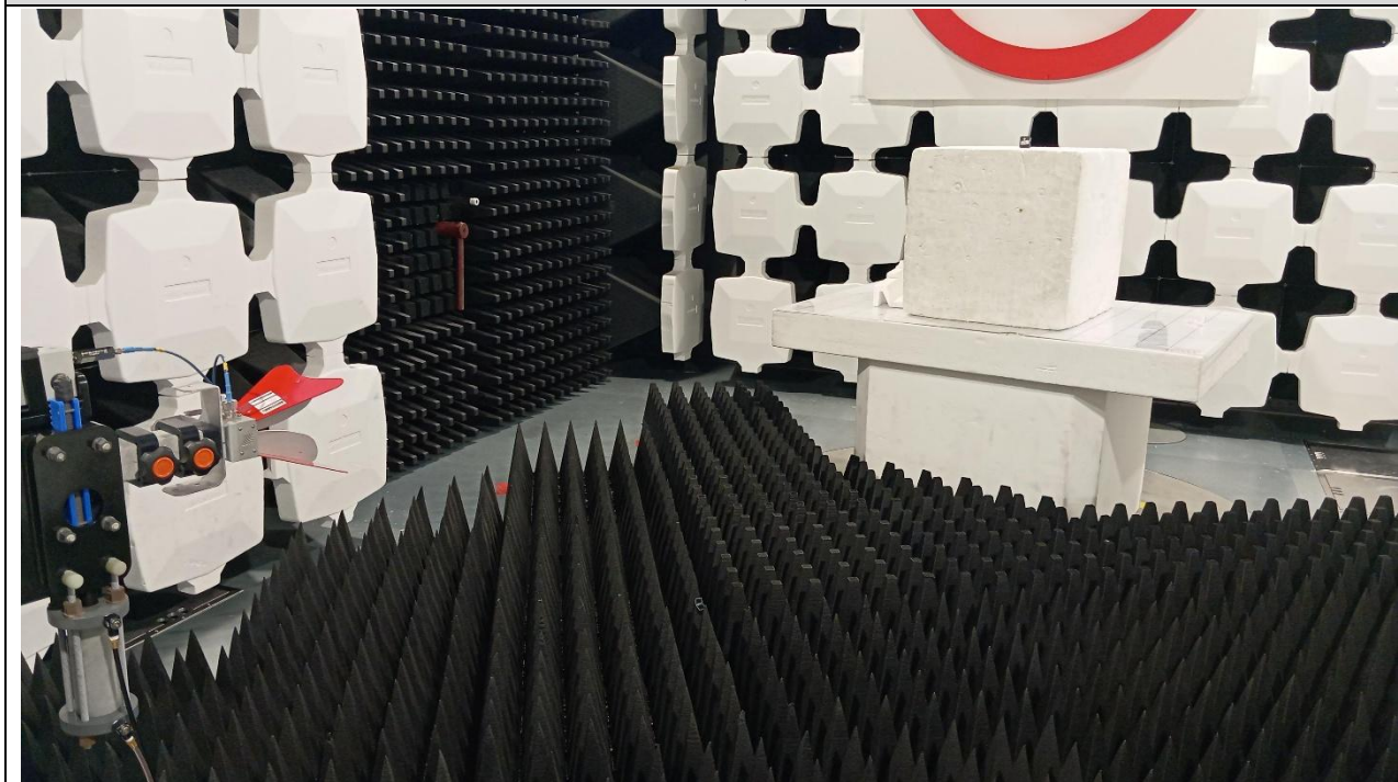
Radiated emission, above 1 GHz
