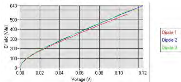
Calibration curves
