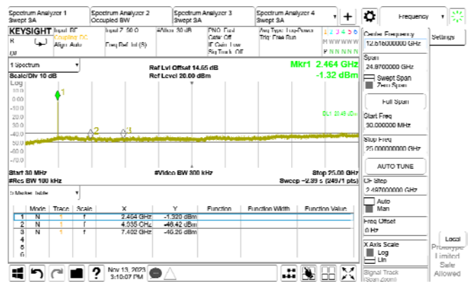
802.11ax_20MHz_WLAN2_2462MHz_RU106_54
