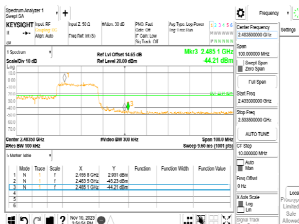
802.11ax_40MHz_WLAN1_2452MHz_RU242_62
