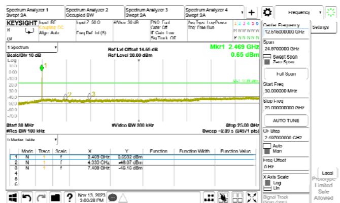
802.11ax_20MHz_WLAN2_2462MHz_RU106_54
