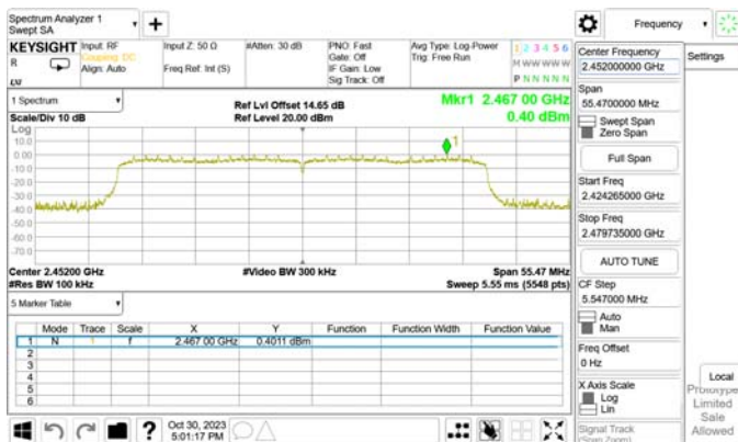
802.11ax_40MHz_WLAN2_2452MHz
