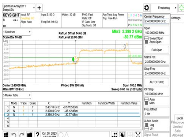
802.11ax_40MHz_WLAN1_2422MHz
