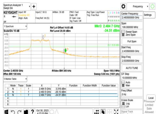
802.11g_20MHz_WLAN1_2462MHz
