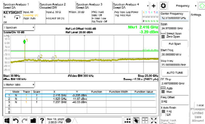
802.11ax_40MHz_WLAN2_2437MHz
