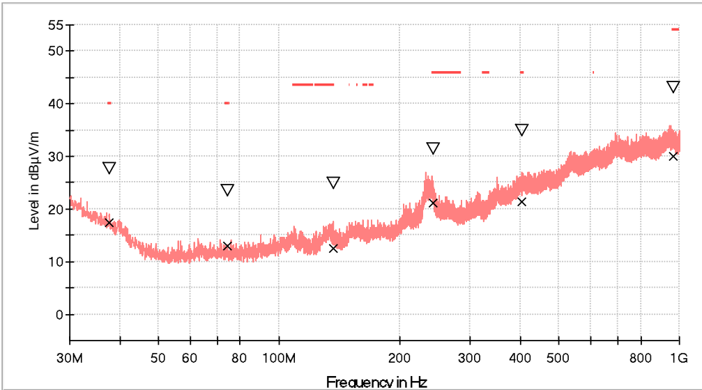
RF_FOC_15.247_E Field_30MHz_1GHz_SAC2
