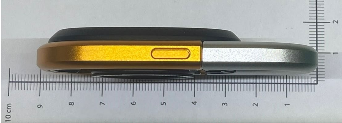
R1T keyfob left view
