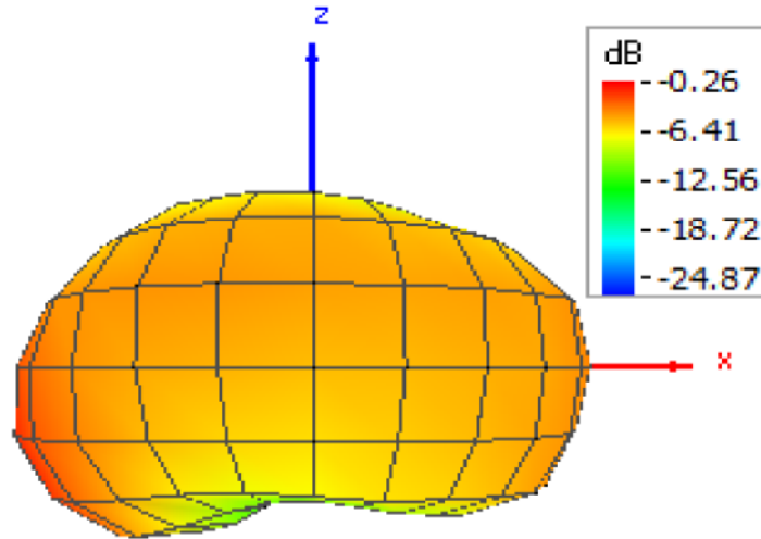
Figure A-3 Pattern at 2402 MHz (Left / Right view)
