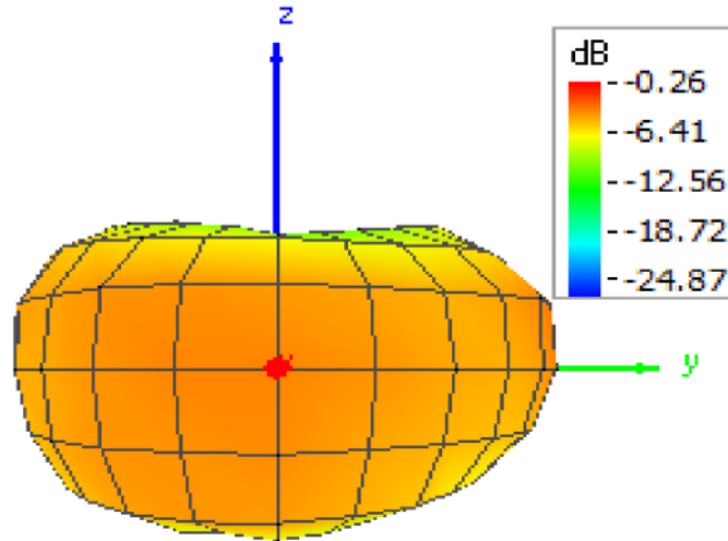
Figure A-2 Pattern at 2402 MHz (Front / Back view)
