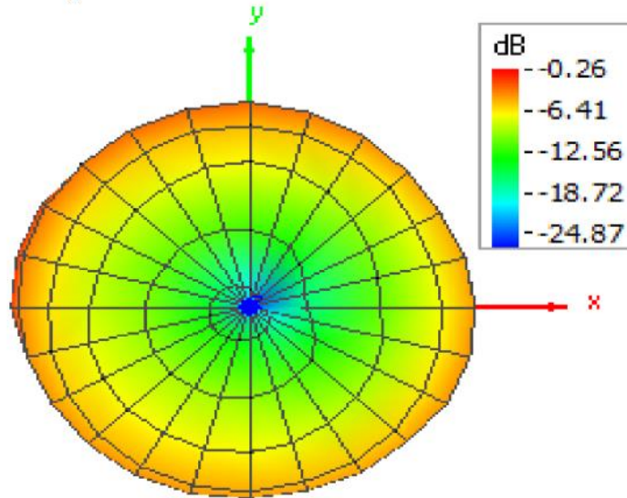
Figure A-1 Pattern at 2402 MHz (Top / Bottom view)
