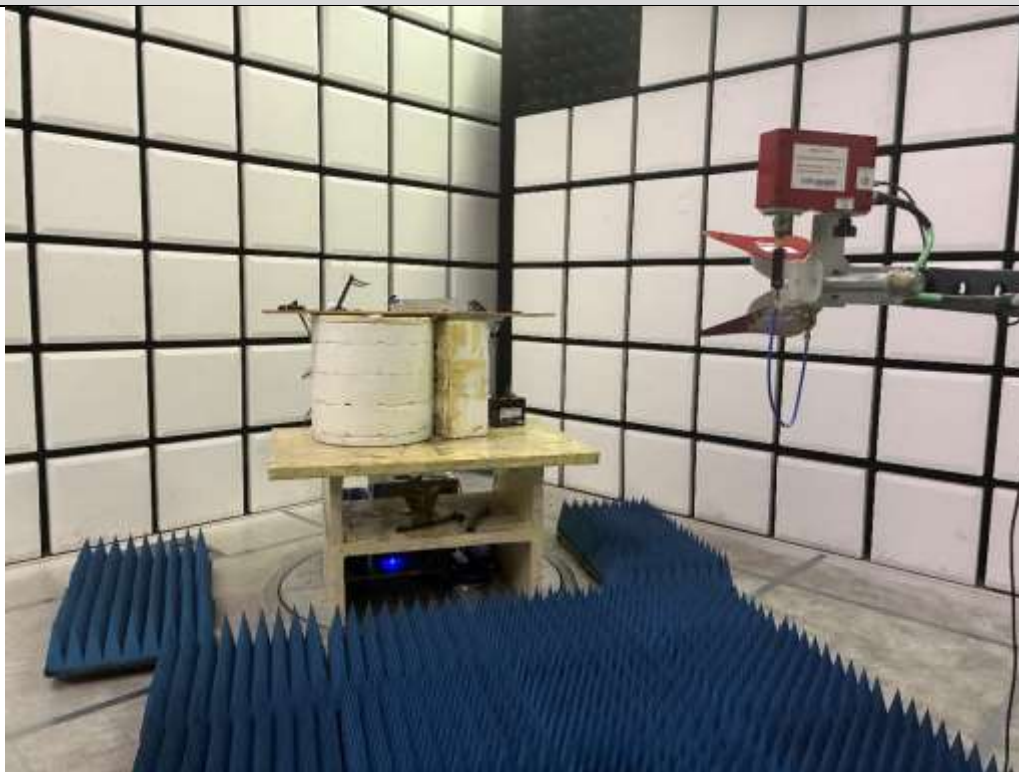
3GHz – 18GHz Rear View
