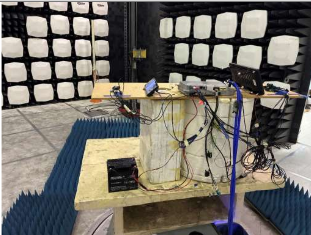
1GHz – 3GHz Rear View
