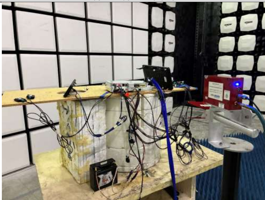
18GHz – 26GHz Rear View
