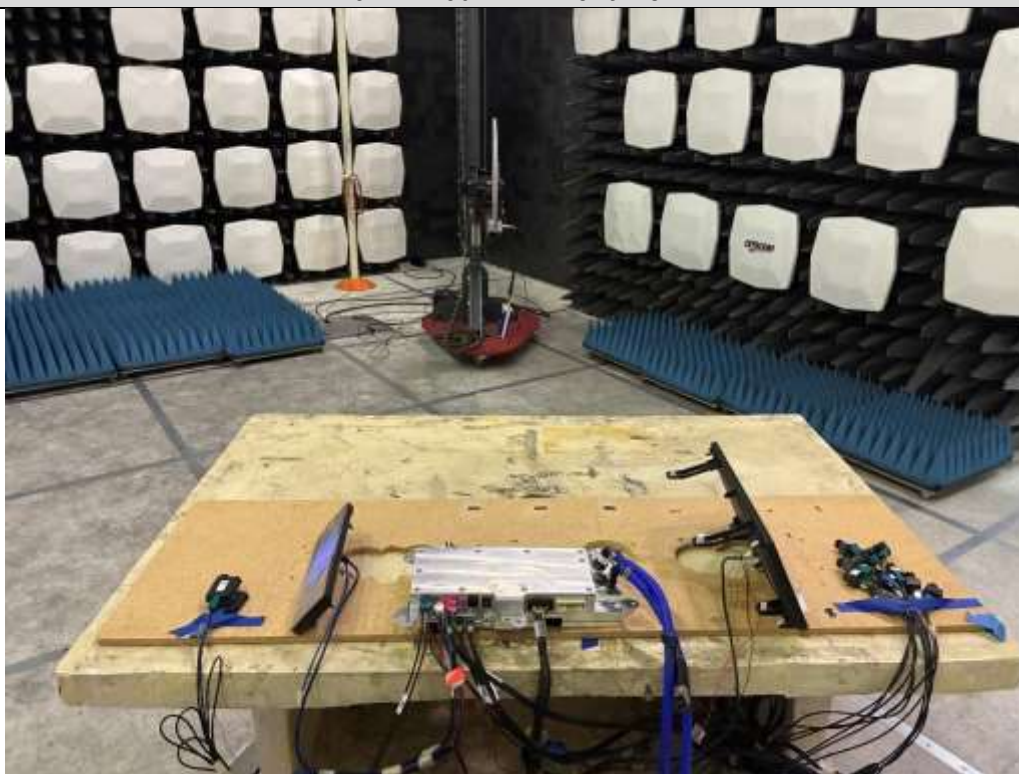
9kHz – 30MHz Rear View
