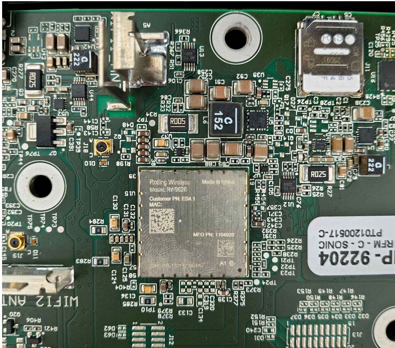
External Photo WiFi Module RW962B
