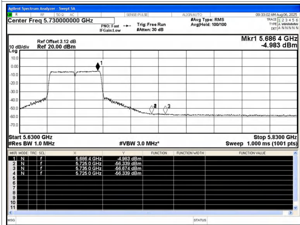
Restrict Band NVNT n40 5670MHz Ant1 Average
