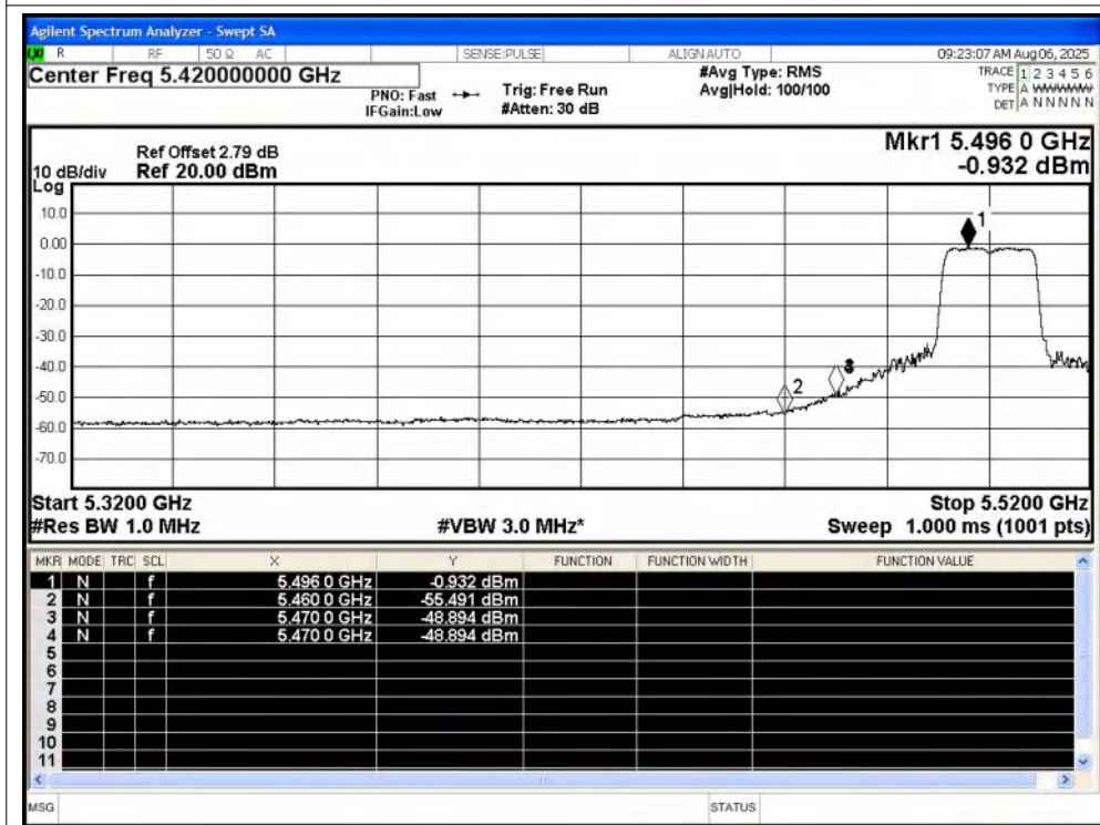
Restrict Band NVNT ac20 5500MHz Ant1 Average
