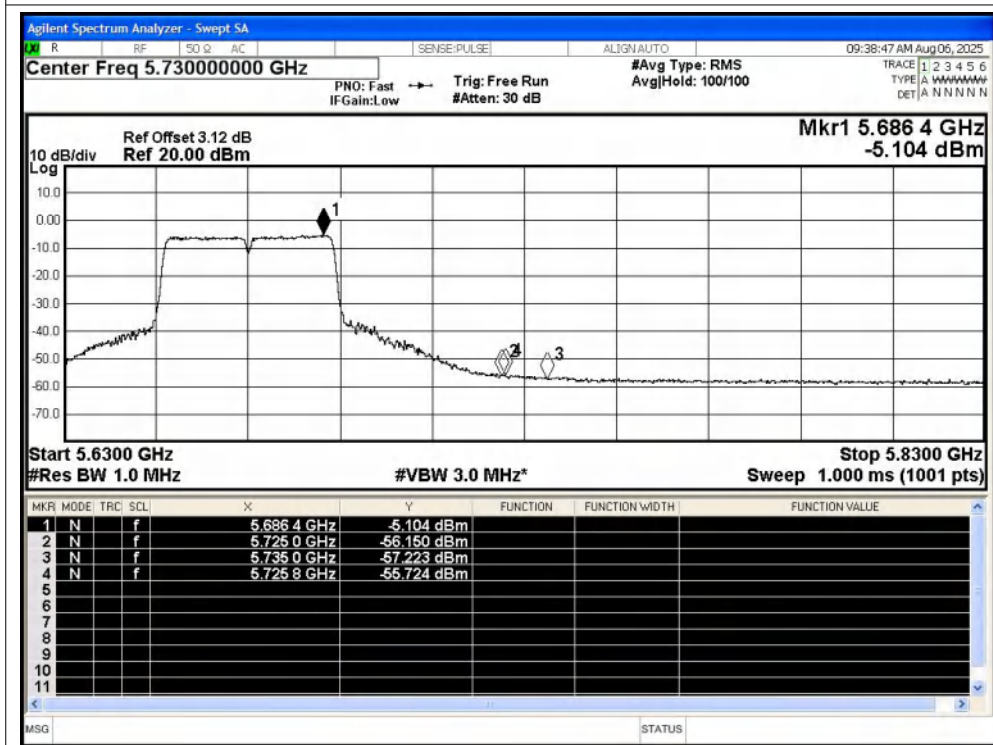
Restrict Band NVNT ac40 5670MHz Ant1 Average
