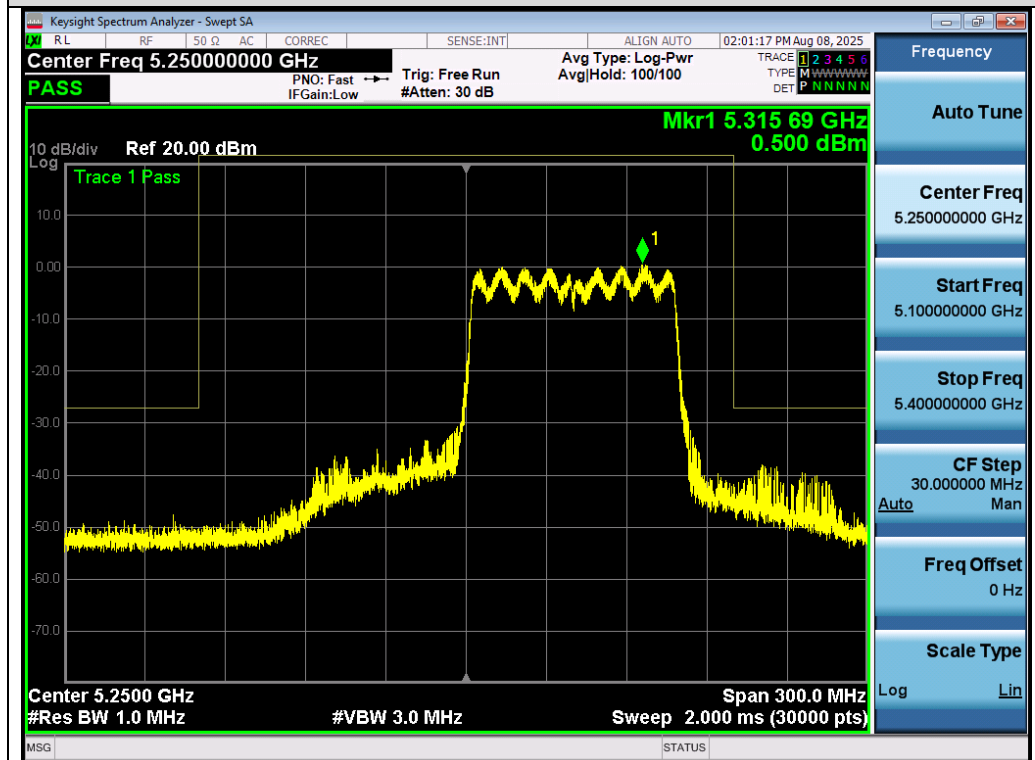
Test_Graph_802.11ac80_ANT1_5290_MCS0_Frequency Band 3
