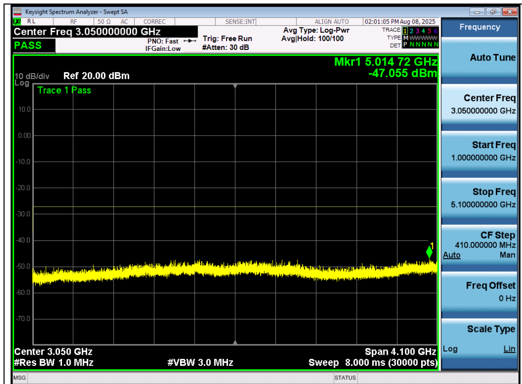
Test_Graph_802.11ac80_ANT1_5290_MCS0_Frequency Band 2
