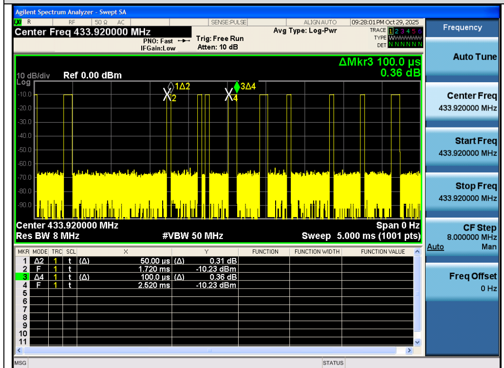
Test_Graph_Pulse_Pulse Type 1_433.92MHz, ASK
