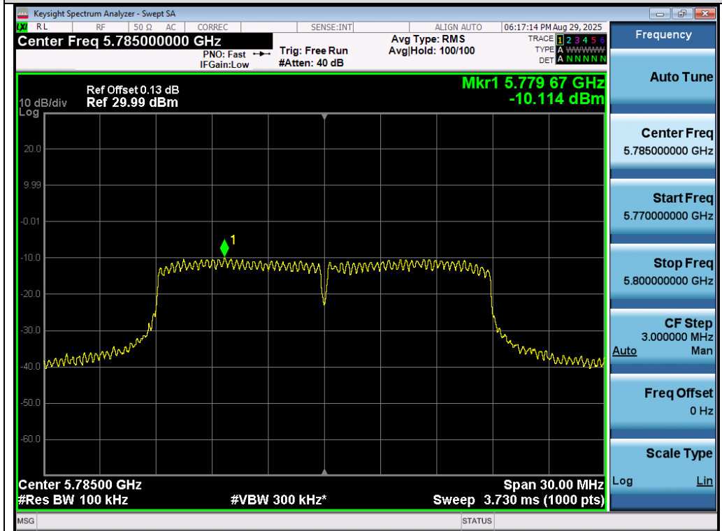
Test_Graph_802.11n20_ANT1_5785_MCS0_PSD
