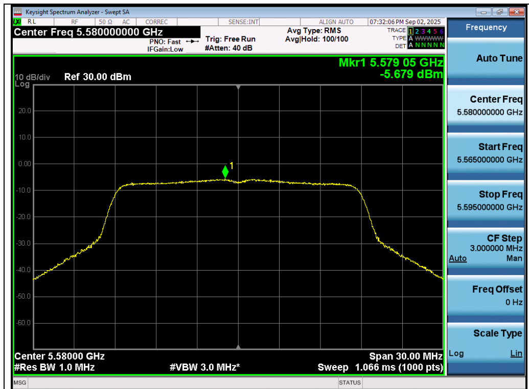
Test_Graph_802.11n20_ANT1_5580_MCS0_PSD
