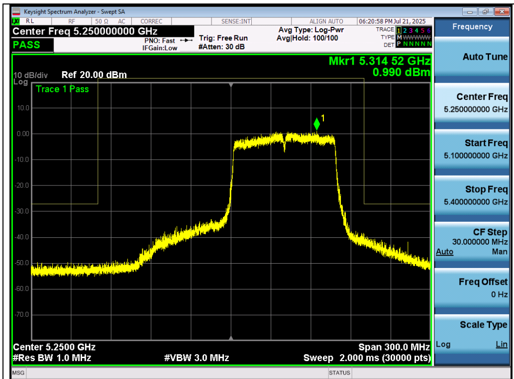
Test_Graph_802.11ac80_ANT1_5290_MCS0_Frequency Band 3
