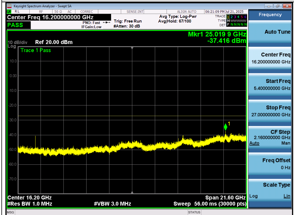
Test_Graph_802.11ac80_ANT1_5290_MCS0_Frequency Band 4
