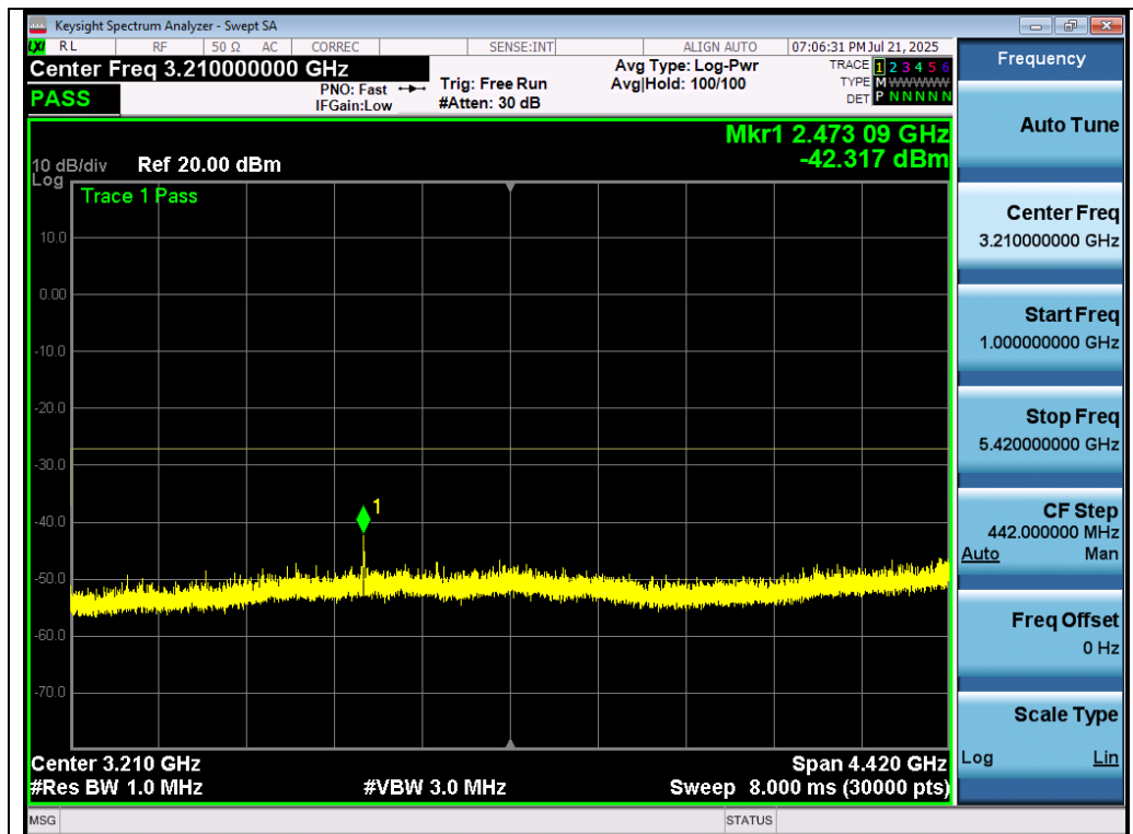
Test_Graph_802.11ac80_ANT1_5530_MCS0_Frequency Band 2
