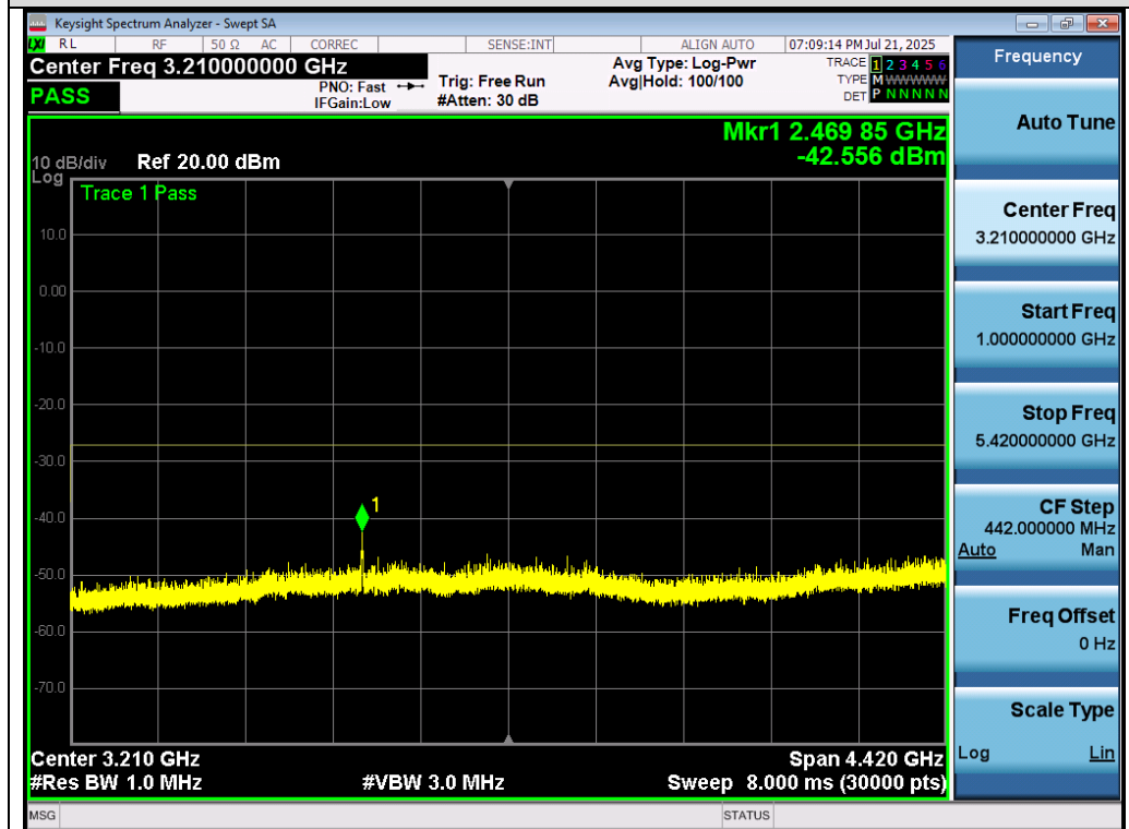
Test_Graph_802.11ac80_ANT1_5610_MCS0_Frequency Band 2
