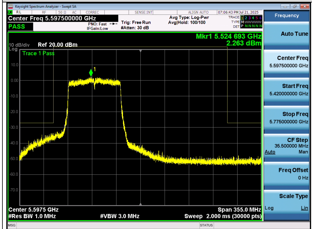
Test_Graph_802.11ac80_ANT1_5530_MCS0_Frequency Band 3
