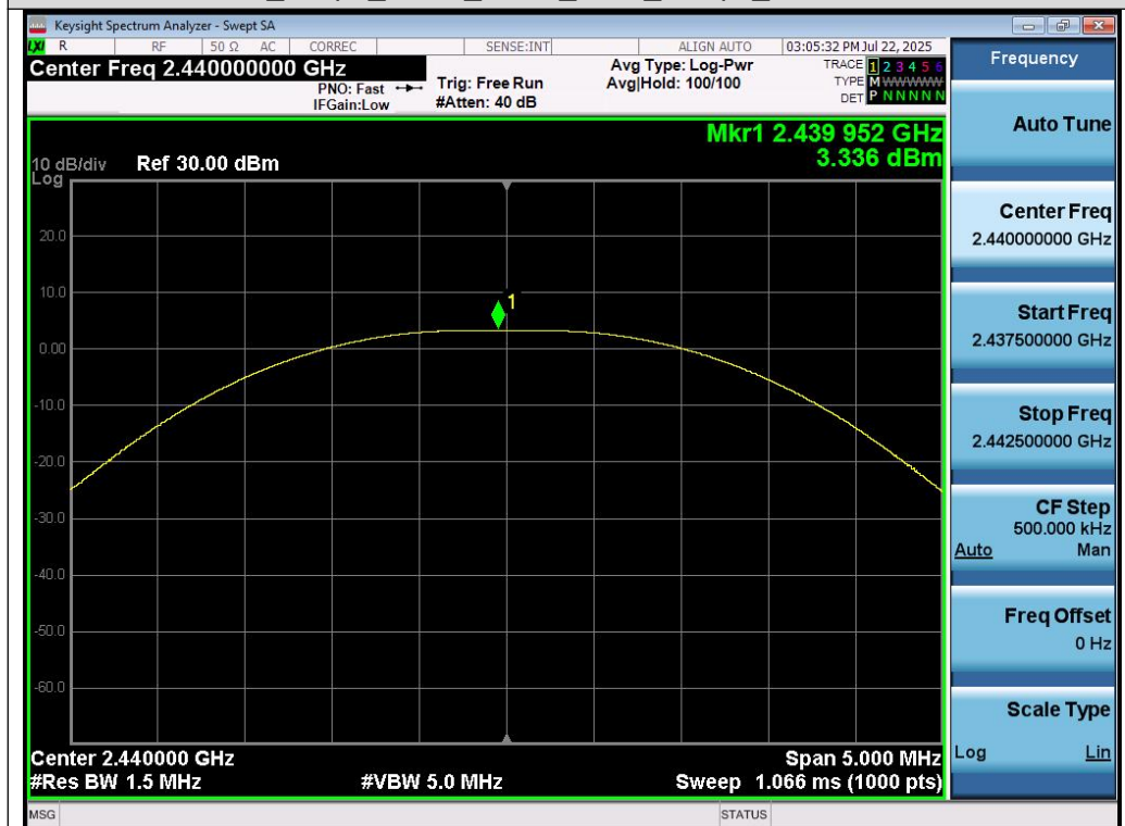
Test Graph LE1M ANT1 2440 1Mbps Peak Power
