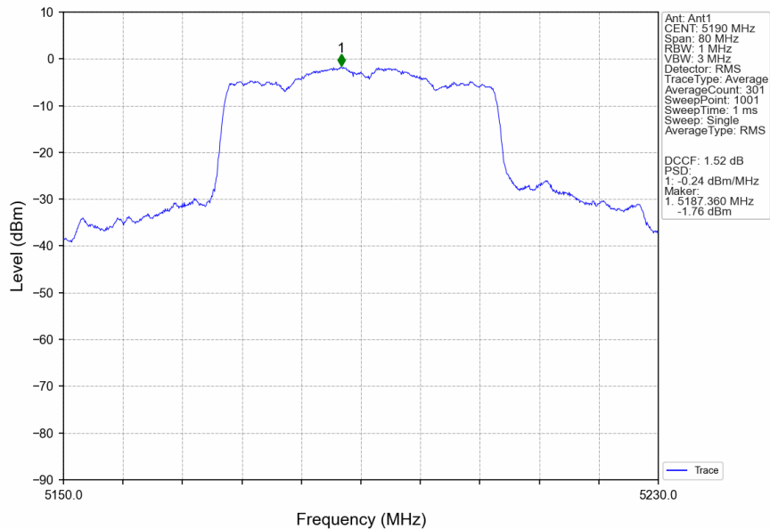
802.11ac(VHT40)_LCH_5190MHz_Ant1_NTNV
