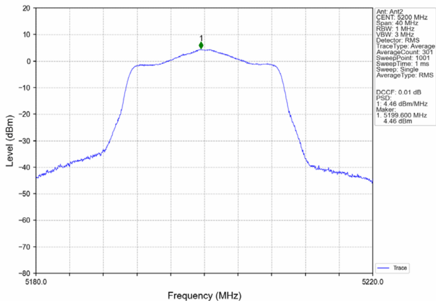
802.11ac(VHT20)_MCH_5200MHz_Ant2_NTNV
