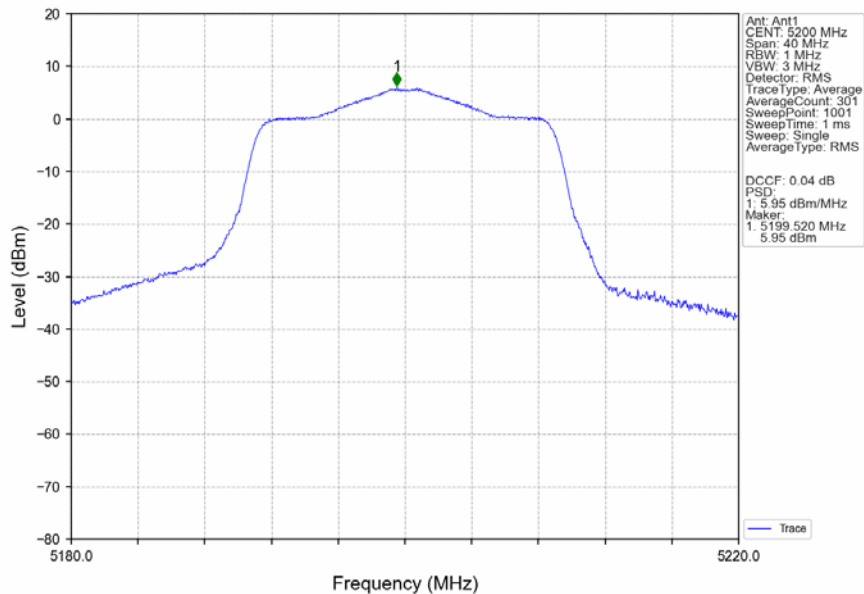
802.11n(HT20)_MCH_5200MHz_Ant1_NTNV
