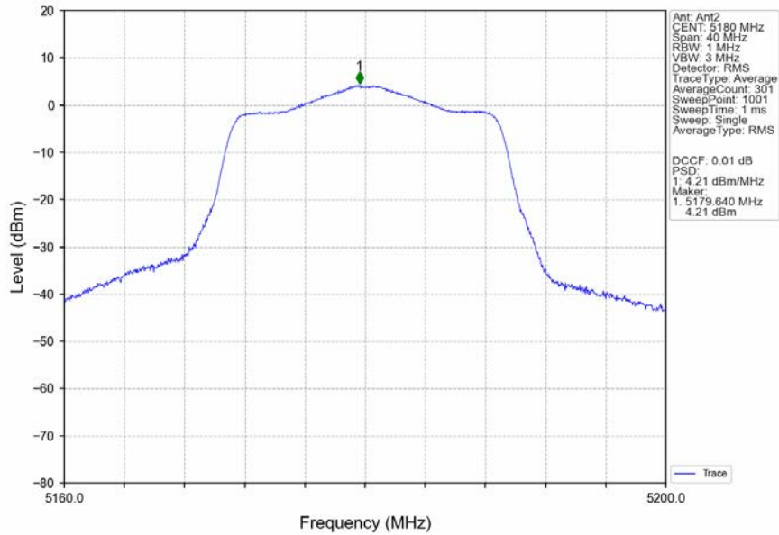
802.11ac(VHT20)_LCH_5180MHz_MIMO_NTNV
