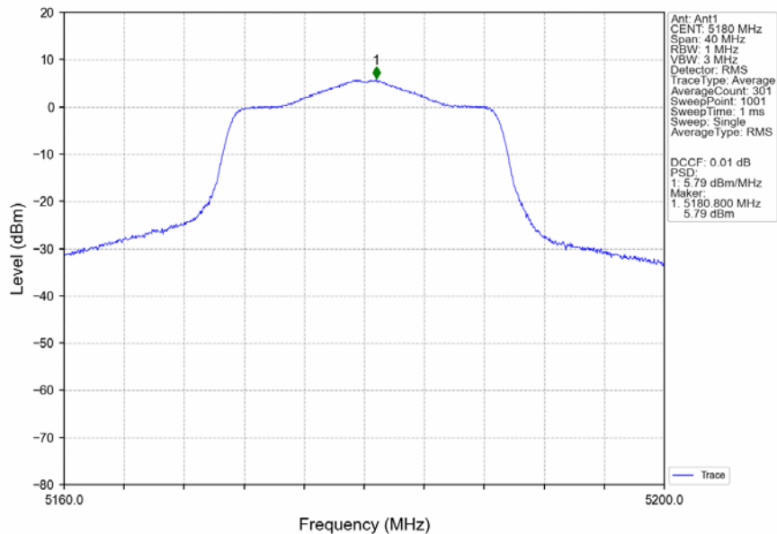
802.11ac(VHT20)_LCH_5180MHz_Ant1_NTNV
