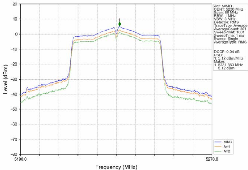
802.11ac(VHT40)_HCH_5230MHz_MIMO_NTNV
