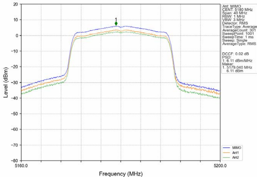
802.11ax(HEW20)_LCH_5180MHz_RU242_Left_MIMO_NTNV
