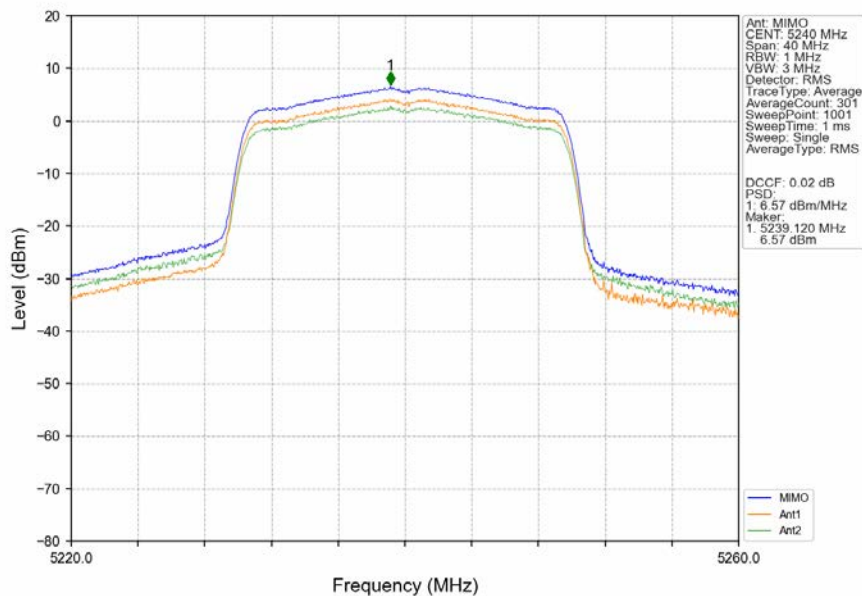
802.11ax(HEW20)_HCH_5240MHz_RU242_Left_MIMO_NTNV
