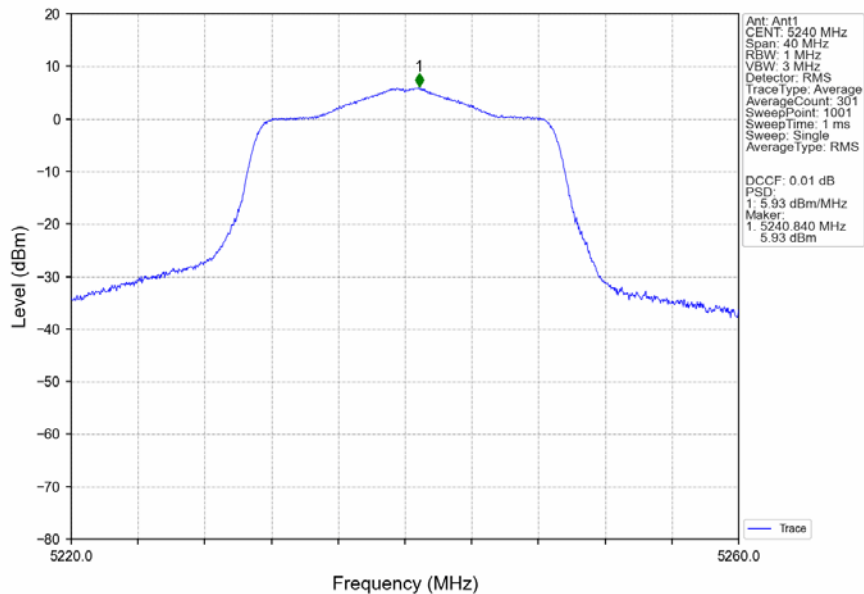
802.11ac(VHT20)_HCH_5240MHz_Ant1_NTNV
