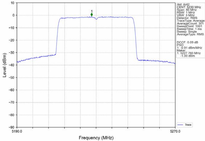
802.11ax(HEW40)_HCH_5230MHz_RU484_Left_MIMO_NTNV
