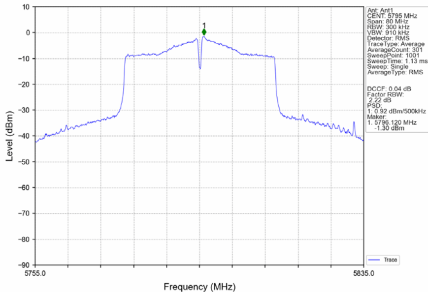
802.11ac(VHT40)_HCH_5795MHz_Ant1_NTNV
