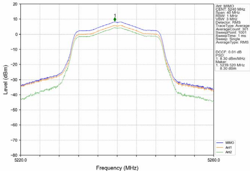
802.11ac(VHT20)_HCH_5240MHz_MIMO_NTNV
