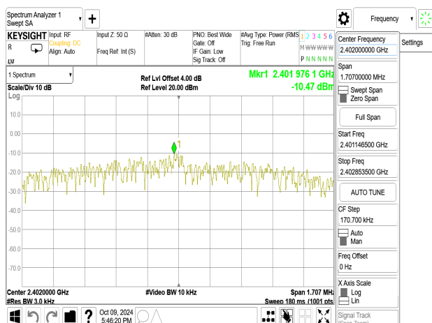
PSD_BLE 2M_LowCH00-2402MHz
