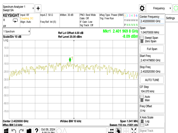
PSD_BLE 1M_LowCH00-2402MHz
