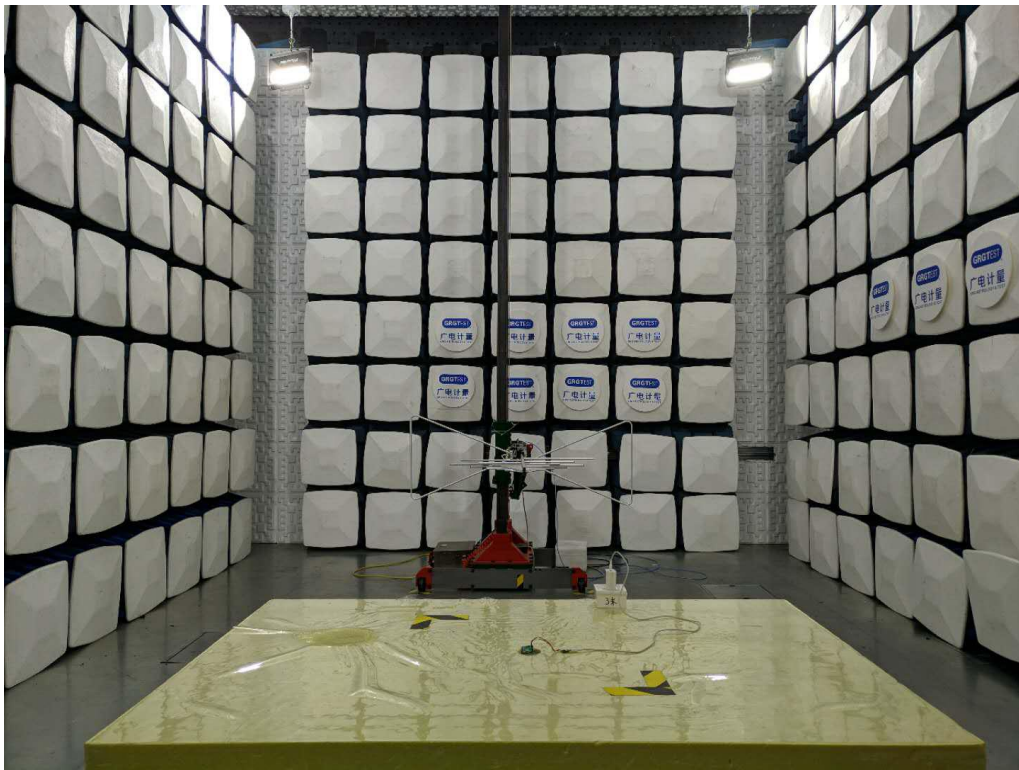
Radiated Spurious Emission Test (Below 1GHz)
