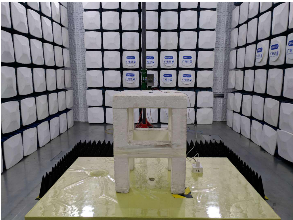
Radiated Spurious Emission Test (Above 1GHz)
