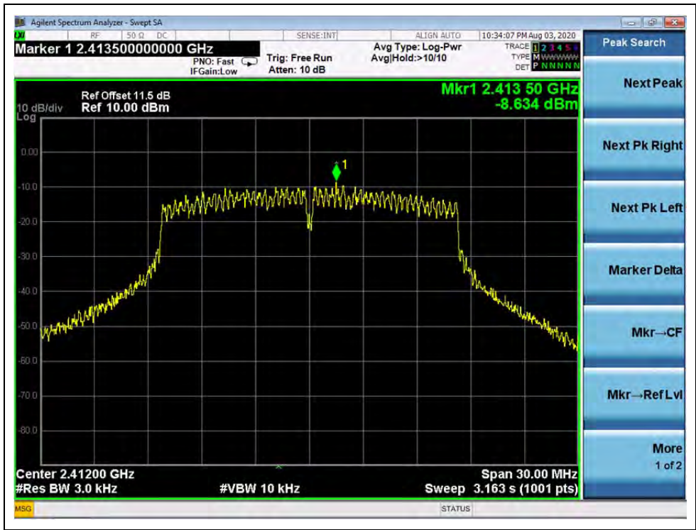
(Channel 1, 802.11g)
