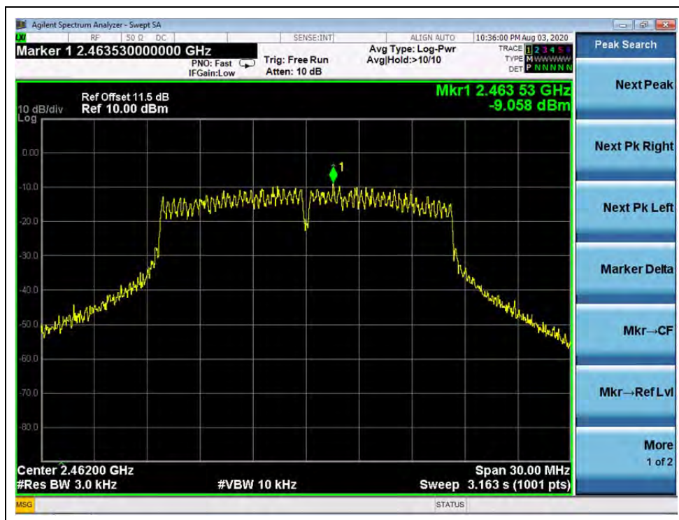
(Channel 11, 802.11g)
