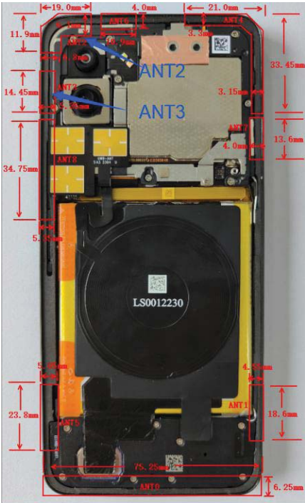
Antenna Photo & Length
