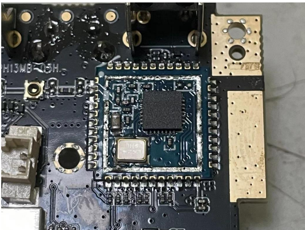
PCB without shield
