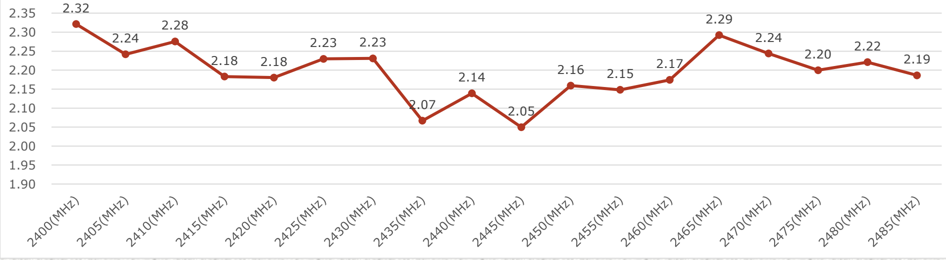
Gain of VPH13
