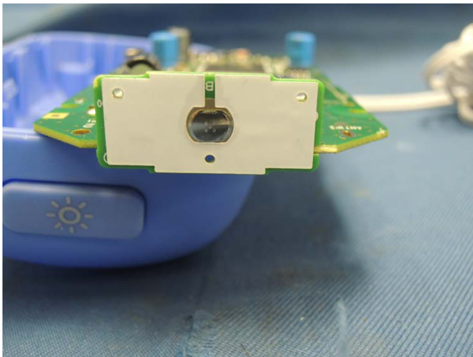
Baby Unit key PCB front side (1)
