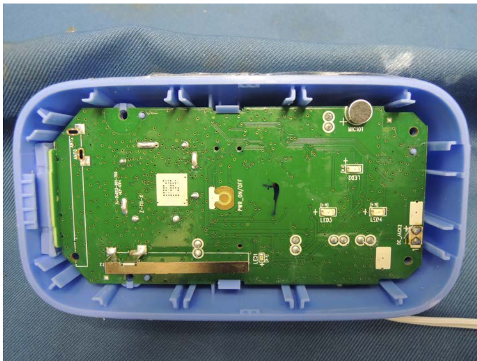
Baby Unit Main PCB solder side
