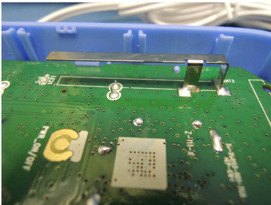
Baby Unit - Antenna
