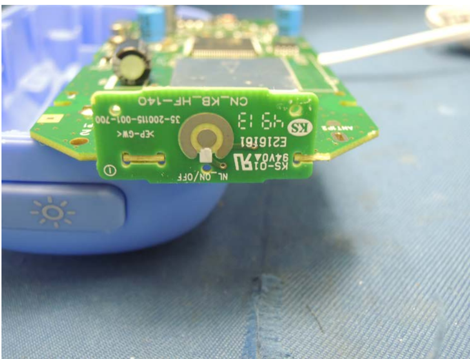
Baby Unit key PCB front side (2)
