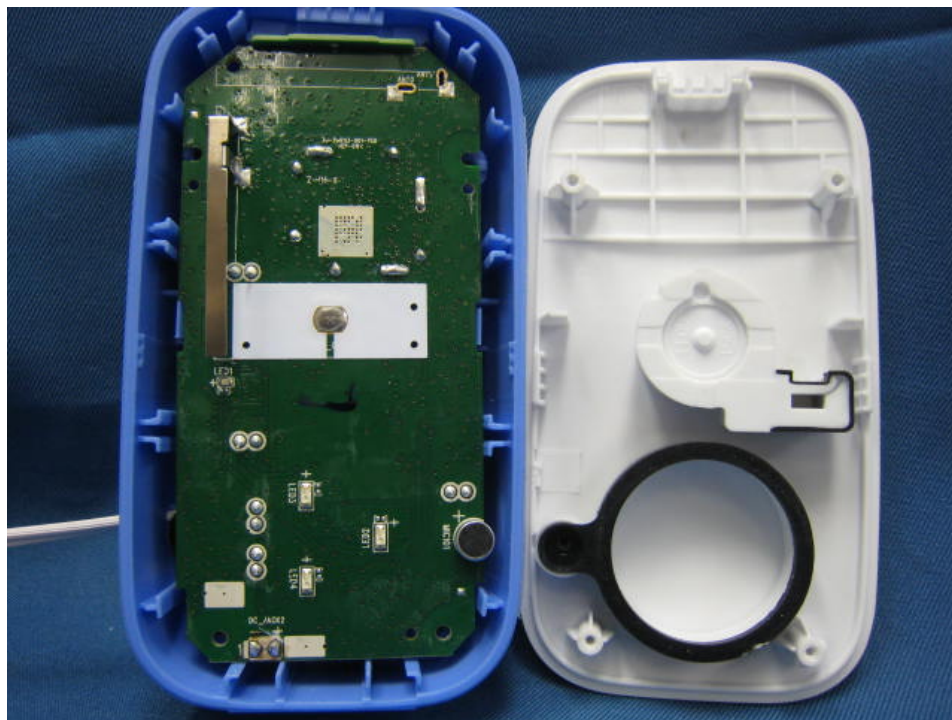
Baby Unit assembly
