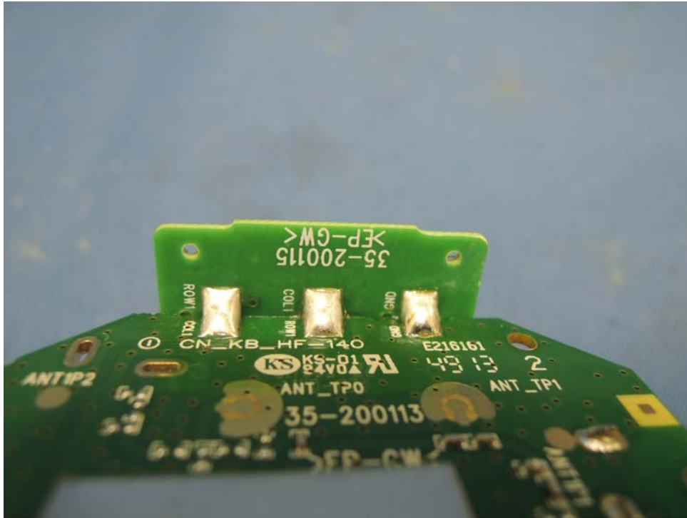
Baby Unit key PCB rear side
