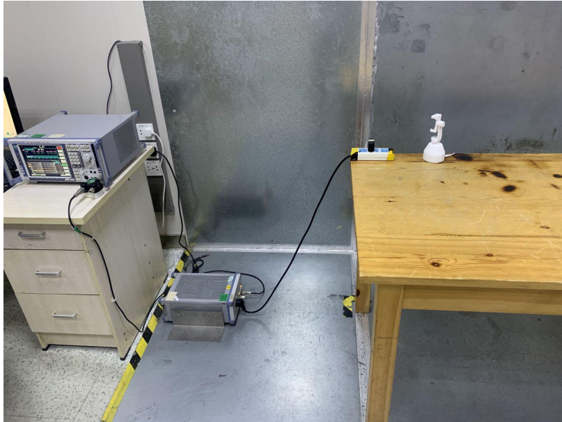
FCC ID: 2AW53-Y1 Conducted Emissions
