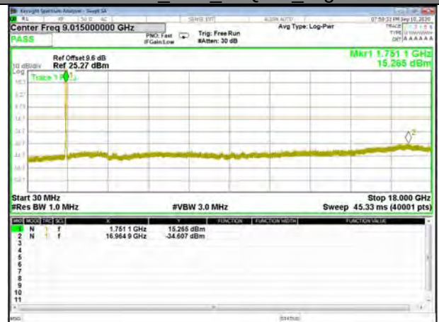
Band4_15M_16QAM_High
