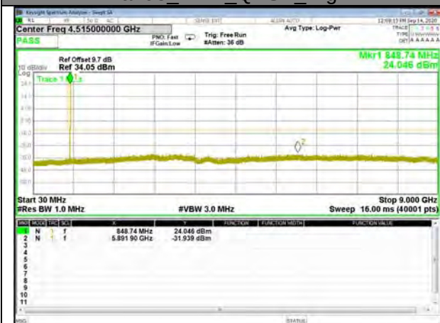
Band5_1.4M_QPSK_High
