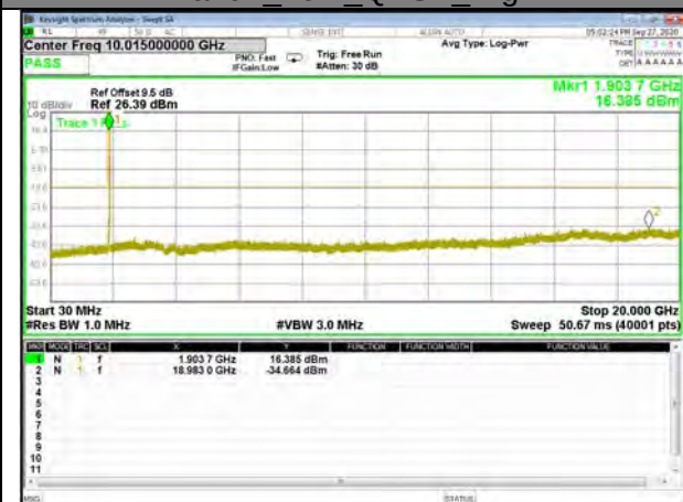
Band2_10M_QPSK_High
