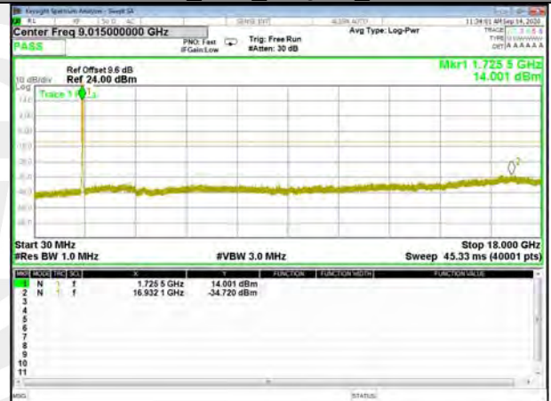
Band4_20M_16QAM_High
