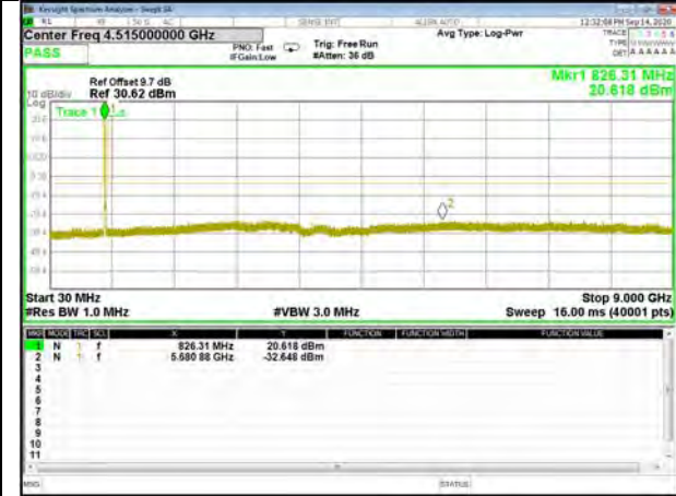
Band5_5M_QPSK_Middle
