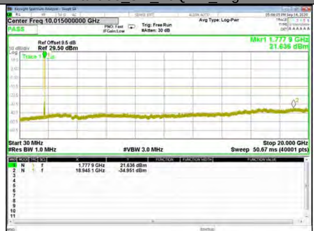
Band66_3M_16QAM_High
