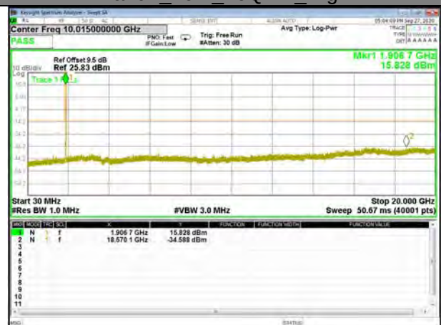
Band2_10M_16QAM_High
