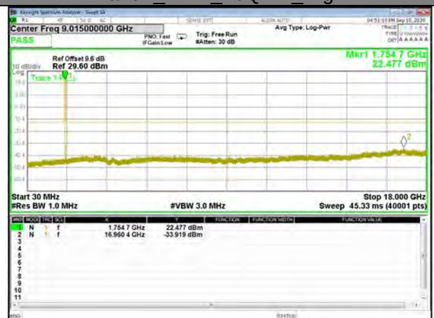
Band4_1.4M_16QAM_High
