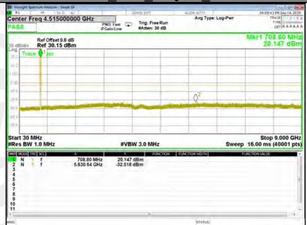
Band12_10M_16QAM_High
