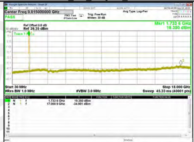
Band4_3M_16QAM_High
