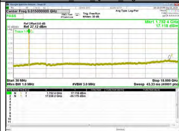
Band4_10M_QPSK_High
