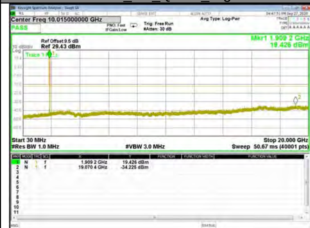
Band2_3M_QPSK_High
