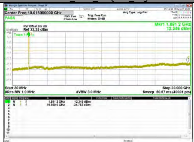
Band2_20M_16QAM_High
