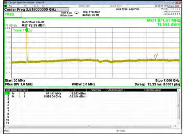
Band71_10M_16QAM_Middle
