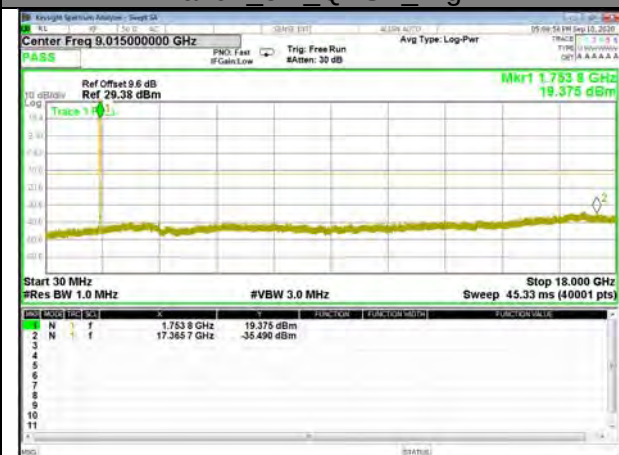
Band4_5M_QPSK_High
