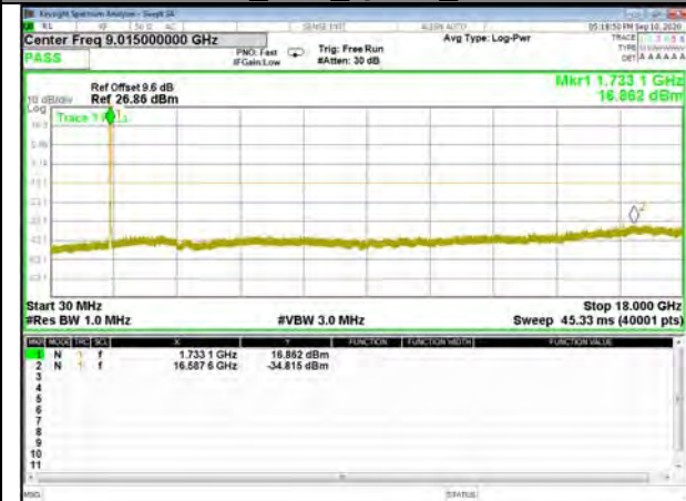
Band4_10M_QPSK_High
