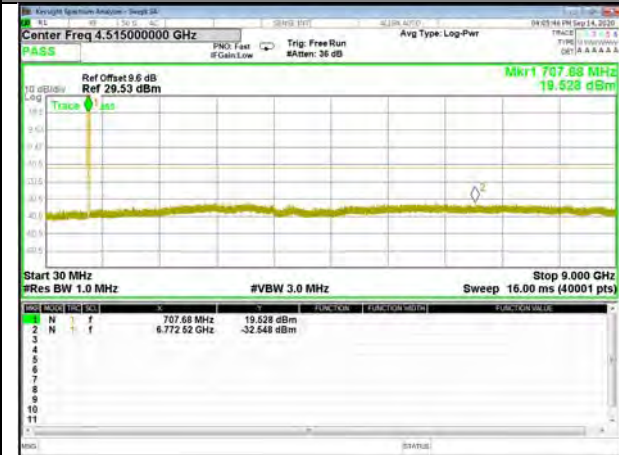
Band12_10M_QPSK_Middle
