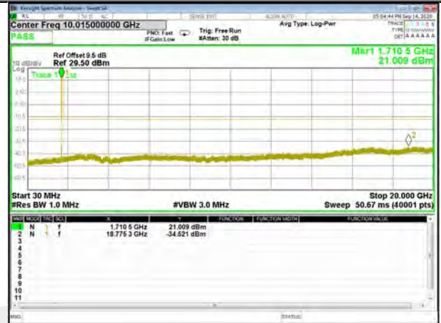
Band66_3M_16QAM_Middle
