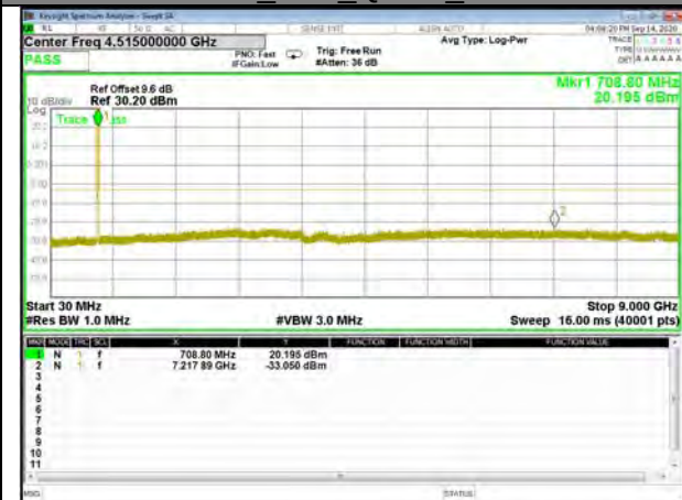
Band12_10M_QPSK_High
