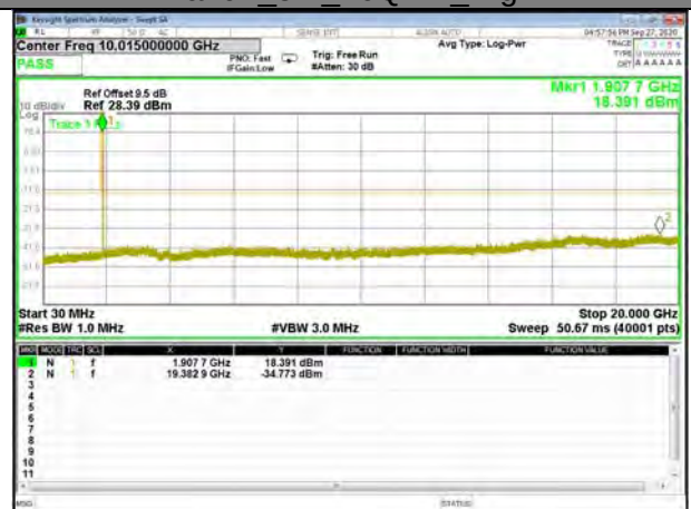
Band2_5M_16QAM_High
