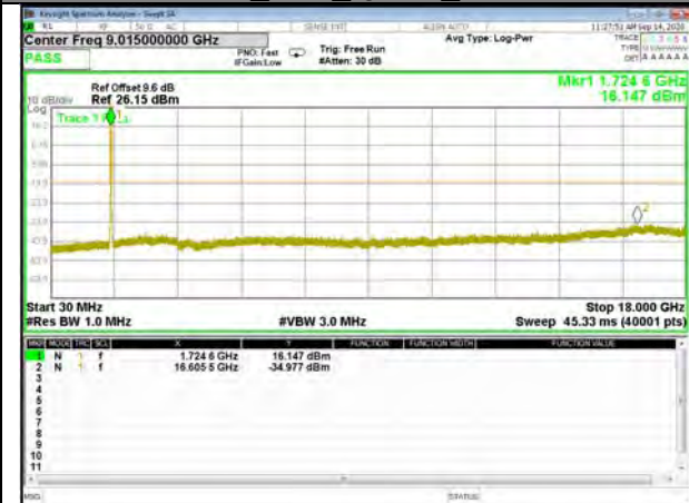
Band4_20M_QPSK_High
