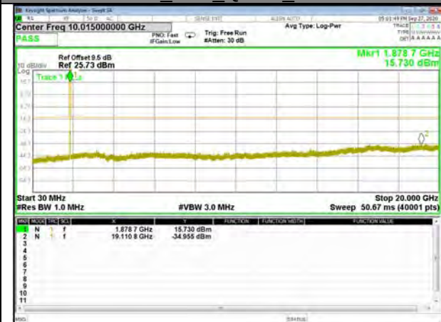
Band2_10M_QPSK_High
