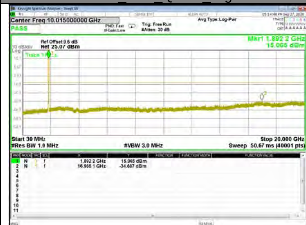
Band2_20M_QPSK_High
