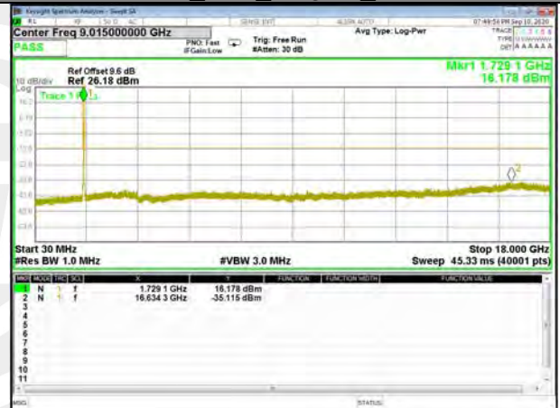
Band4_15M_16QAM_High
