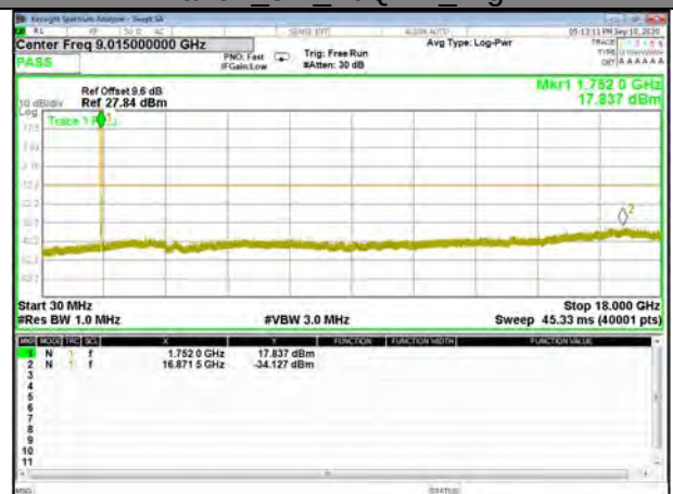
Band4_5M_16QAM_High
