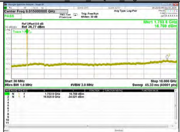
Band4_10M_16QAM_High
