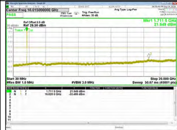
Band66_3M_QPSK_Middle
