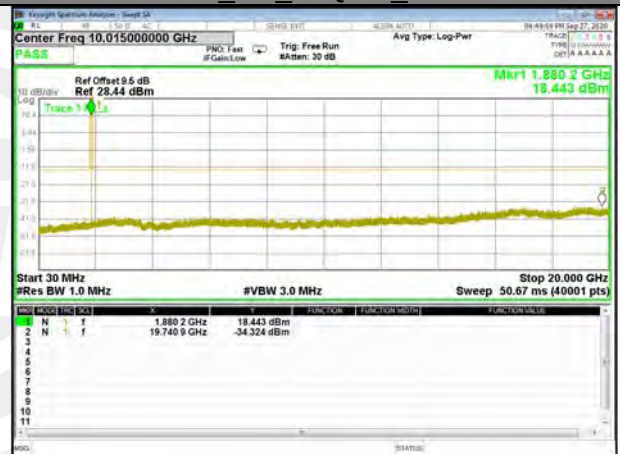
Band2_3M_16QAM_High
