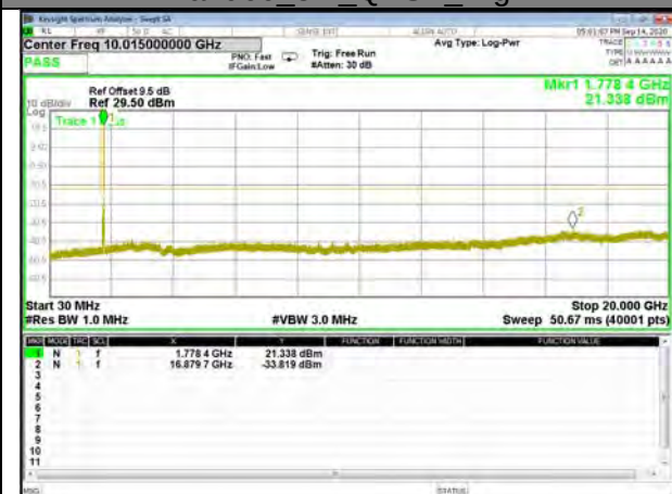
Band66_3M_QPSK_High
