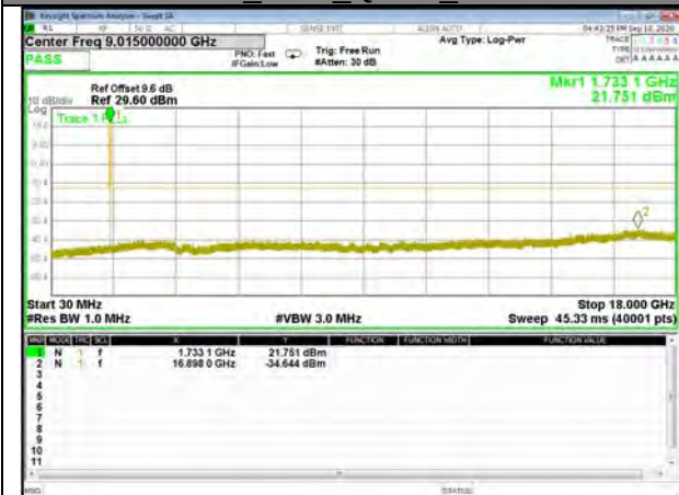
Band4_1.4M_QPSK_High
