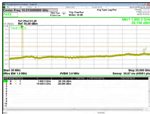
GPRS1900 Low Conducted Spurious
