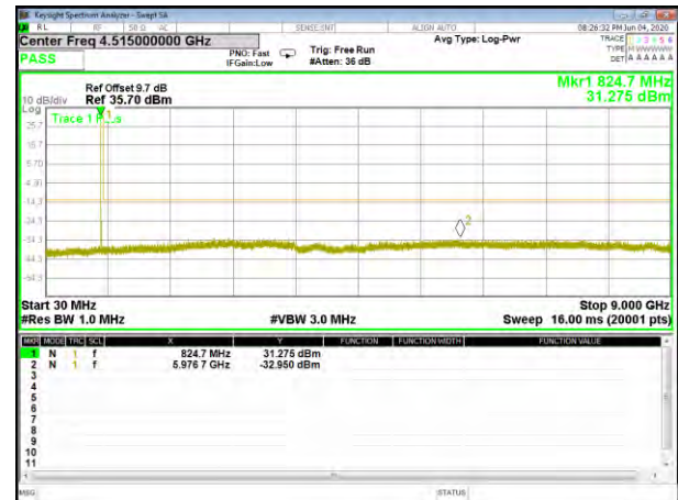
GPRS850 Low Conducted Spurious
