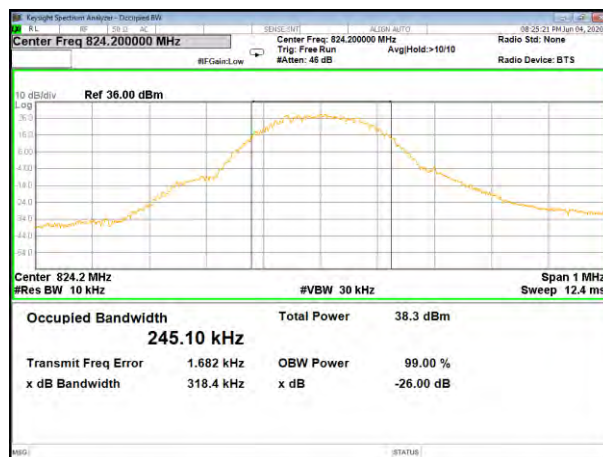
GPRS850 Low 26BW and 99%
