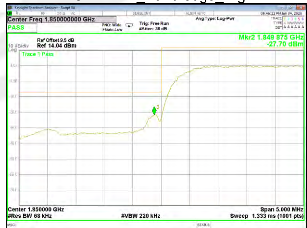
HSDPA B2_Band edge_Low
