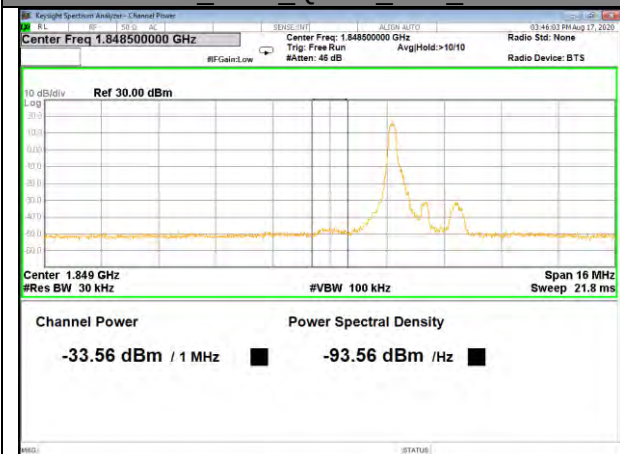
Band2_1.4M_QPSK_Low_Full-RB
