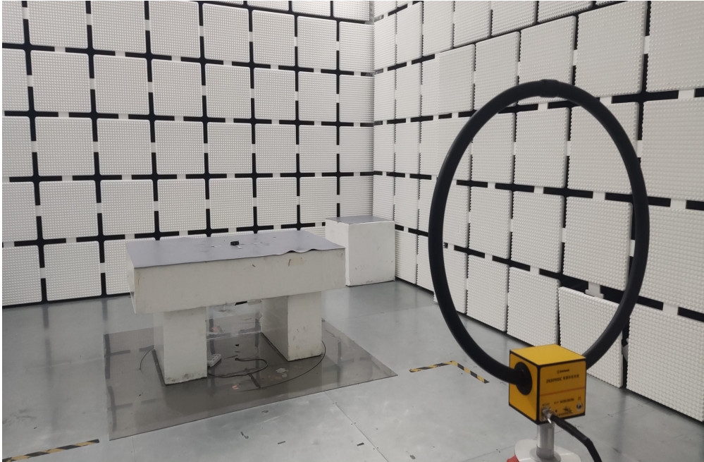
Radiated Emissions for 9KHz~30MHz
