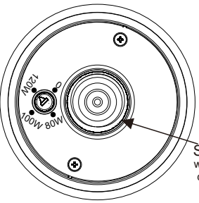
Single CCT80-120W
