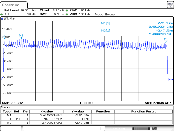
2DH1_Hopping
