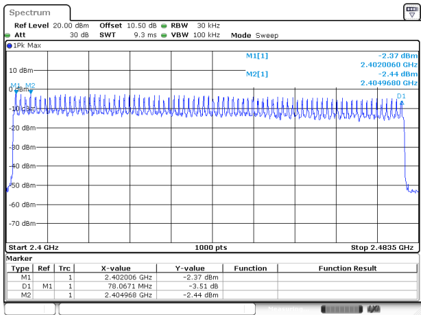
3DH1_Hopping
