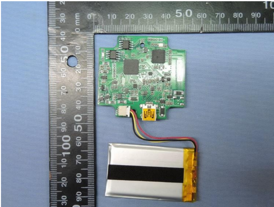
Main board
