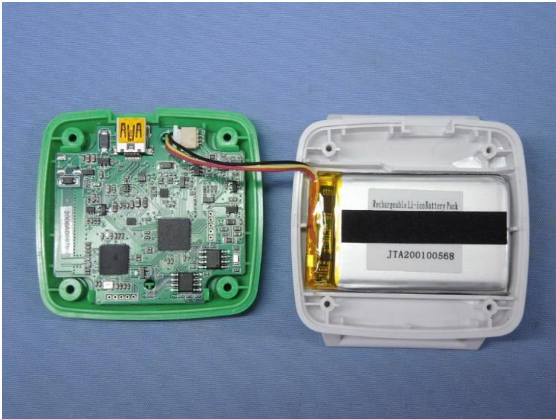
Main board
