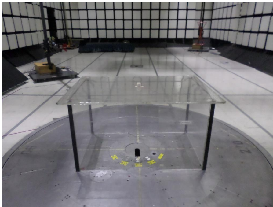
Figure 6: Radiated Spurious Emissions, Below 1GHz - Setup Rear View
