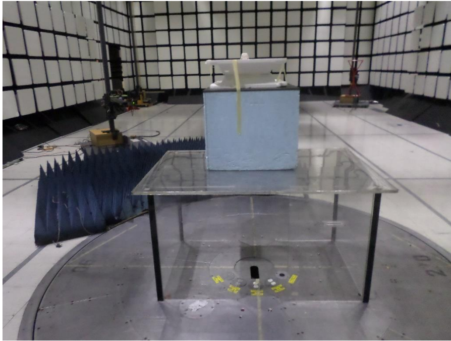
Figure 9: Radiated Spurious Emissions, Above 1GHz - Setup Rear View
