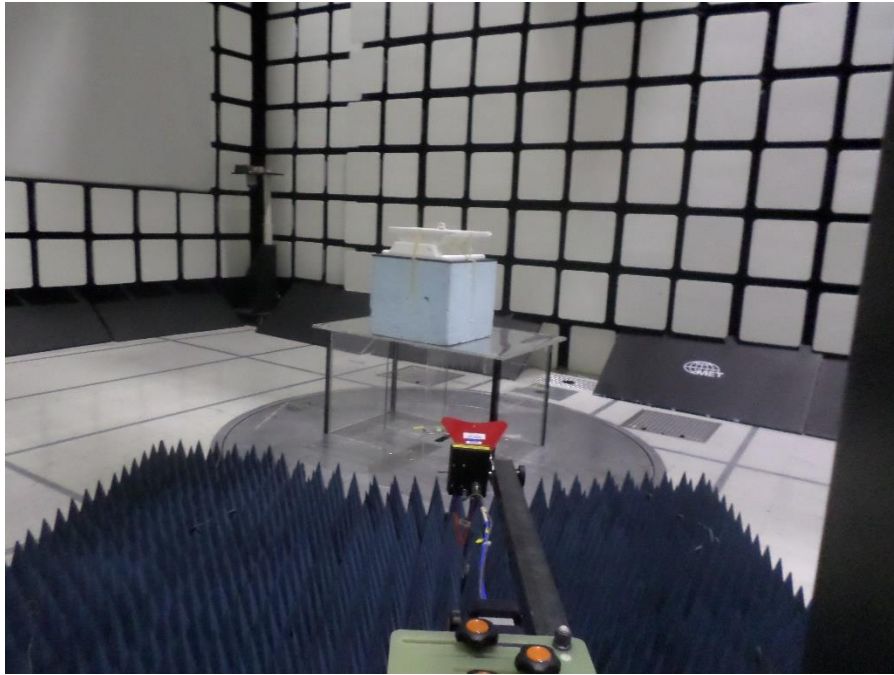
Figure 7: Radiated Spurious Emissions, Above 1GHz - Setup Antenna View
