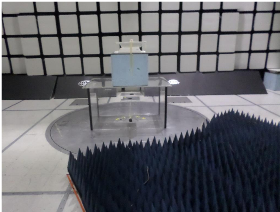
Figure 8: Radiated Spurious Emissions, Above 1GHz - Setup Front View
