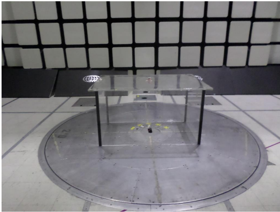
Figure 5: Radiated Spurious Emissions, Below 1GHz - Setup Front View
