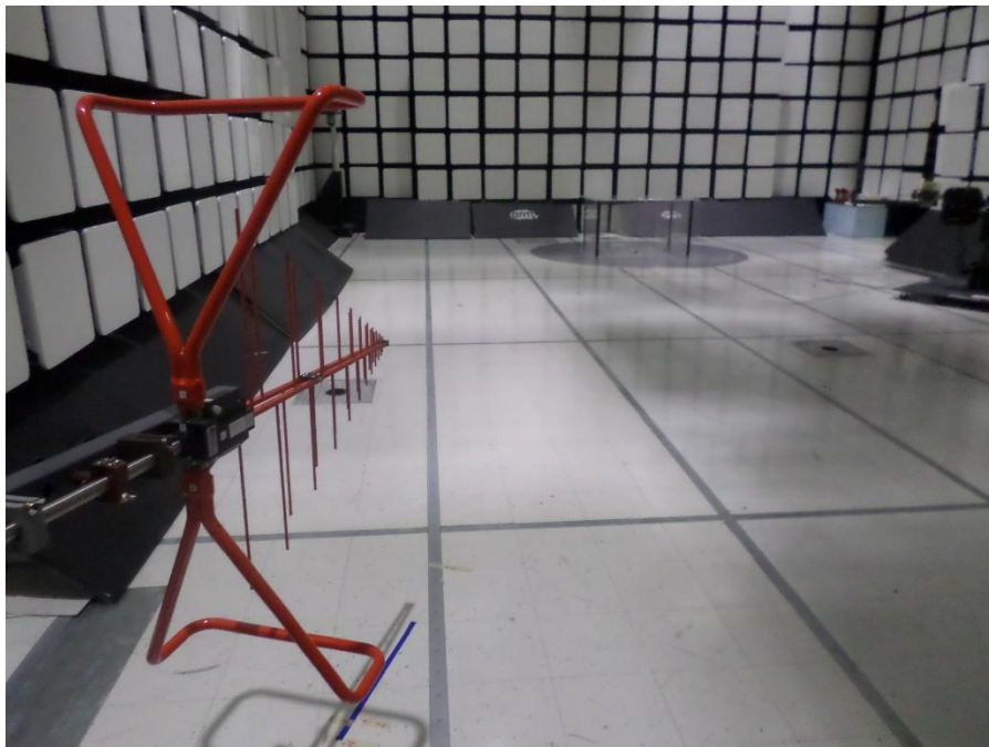
Figure 4: Radiated Spurious Emissions, Below 1GHz - Setup Antenna View
