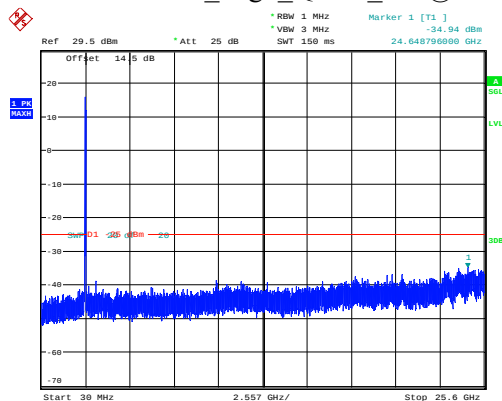
20MHz_High_QPSK_100@0
