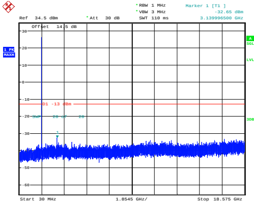
15MHz_Low_QPSK_1@0
