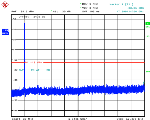
15MHz_High_QPSK_1@0
