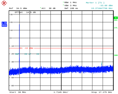
15MHz_Low_QPSK_75@0
