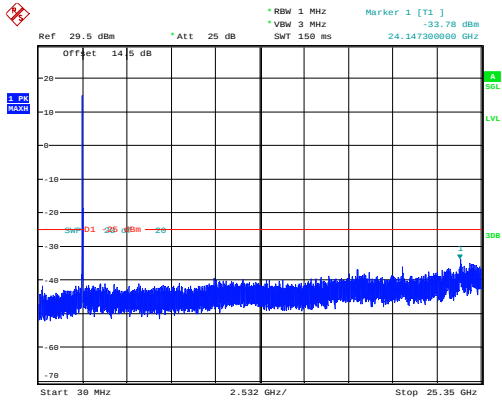
15MHz_Middle_QPSK_75@0
