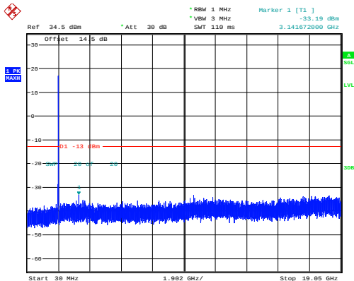
10MHz_High_QPSK_50@0
