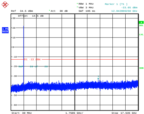
3MHz_High_QPSK_15@0
