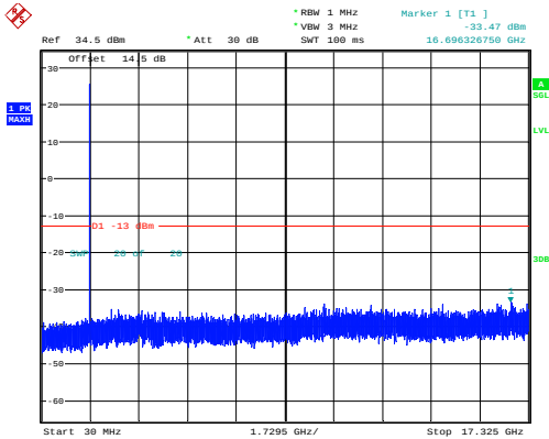
3MHz_Middle_QPSK_1@0
