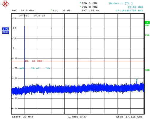
3MHz_Low_QPSK_15@0
