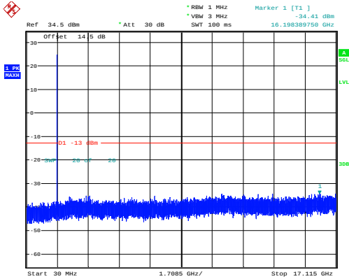
3MHz_Low_QPSK_1@0
