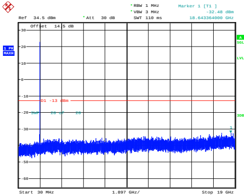
20MHz_High_QPSK_1@0
