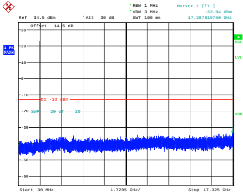
3MHz_Middle_QPSK_15@0
