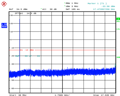
3MHz_High_QPSK_1@0
