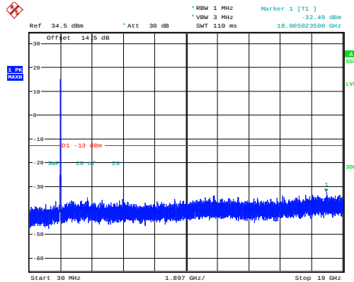
20MHz_High_QPSK_100@0
