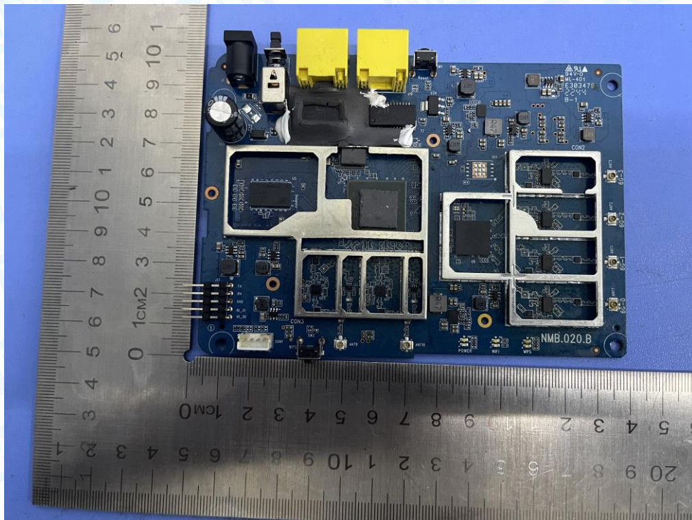
Photo 20 Appearance of PCB
