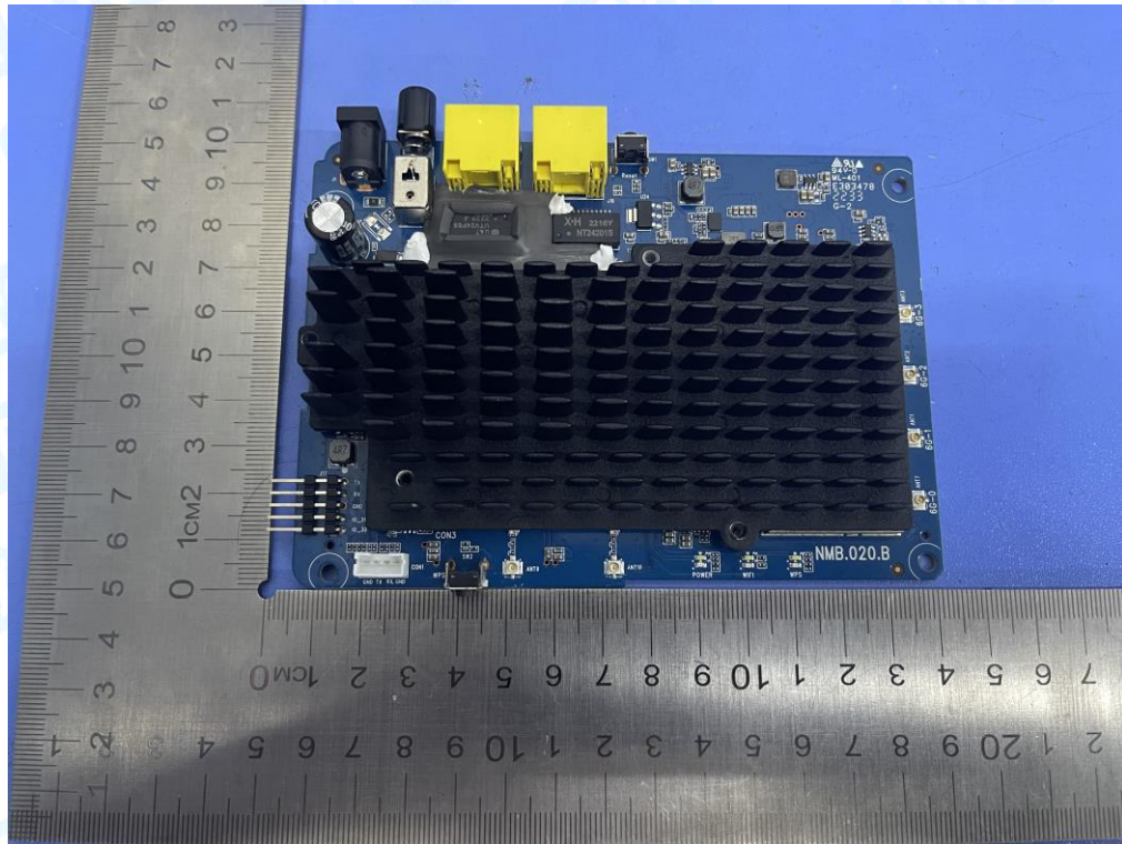
Photo 19 Appearance of PCB
