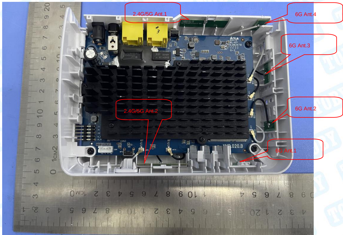
Photo 18 Appearance of PCB
