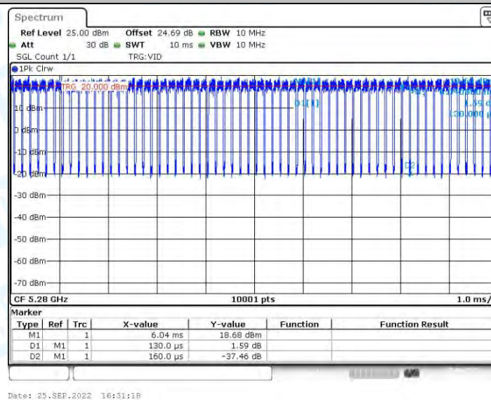
11AC20-SDM_Ant2_5280
