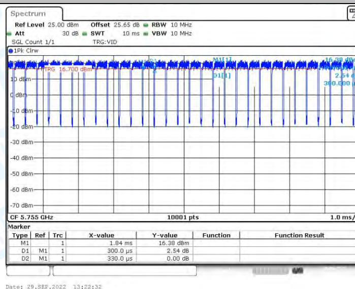
11AX40-SDM_Ant2_5755
