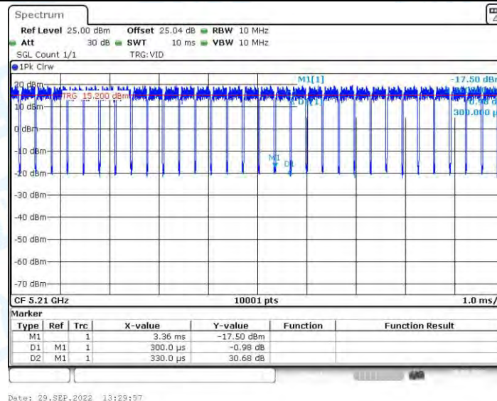
11AX80-SDM_Ant2_5210
