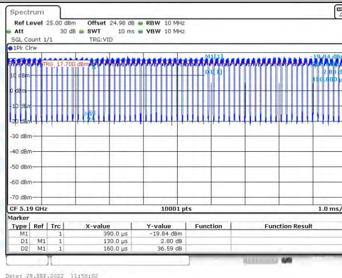
11AC40-SDM_Ant2_5190
