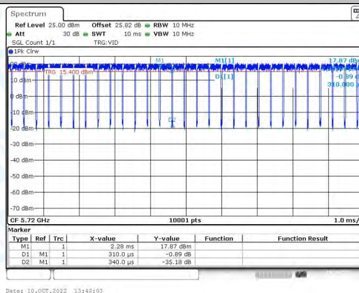
11AX20-SDM_Ant2_5720
