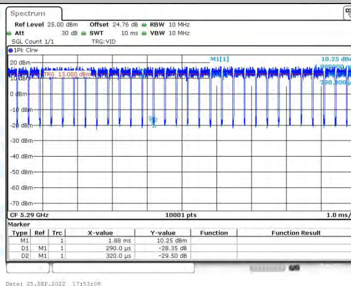
11AX80-SDM_Ant2_5290
